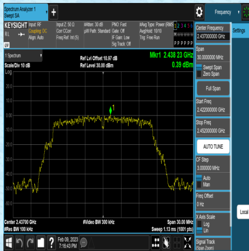
11G-Ant1-2437-Reference-0.39
