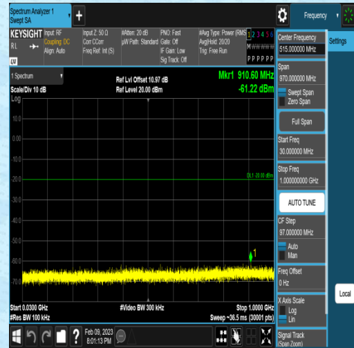
11G-Ant2-2437-30~1000-0.00
