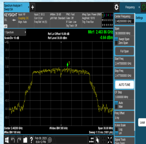
11G-Ant2-2462-Reference--0.64
