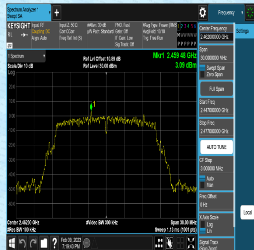
11G-Ant1-2462-Reference-3.09
