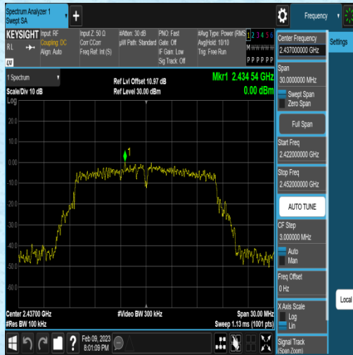
11G-Ant2-2437-Reference-0.00
