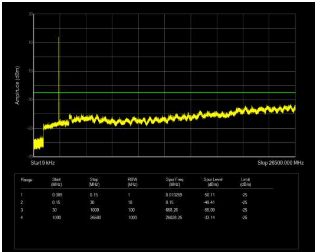
Band41 16QAM BW=15MHz Channel=40165 RB Size=75 Position=#0
