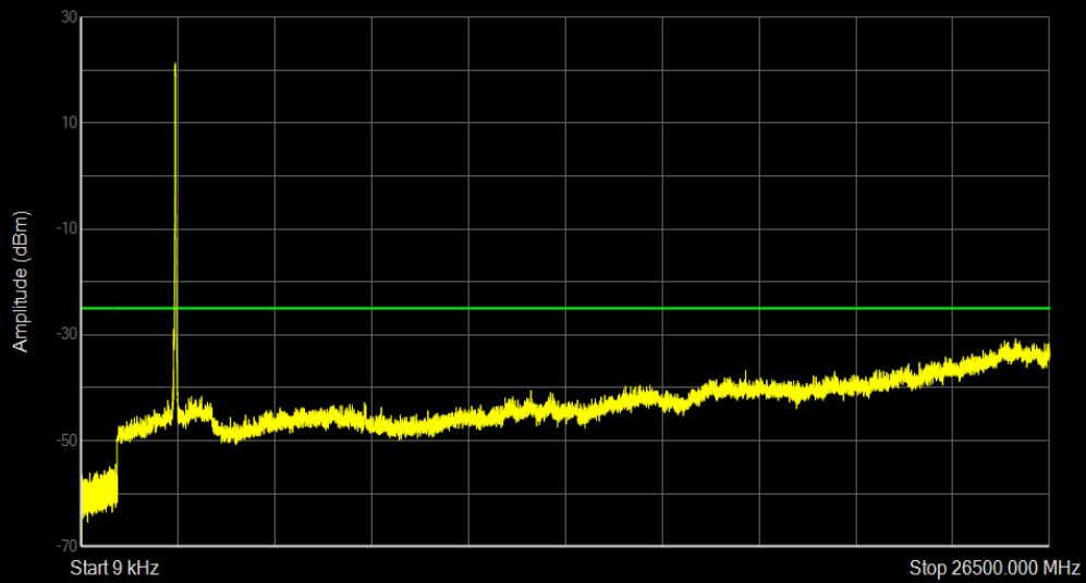
Band41(2535-2655) QPSK BW=20MHz Channel=40640 RB Size=100 Position=#0
