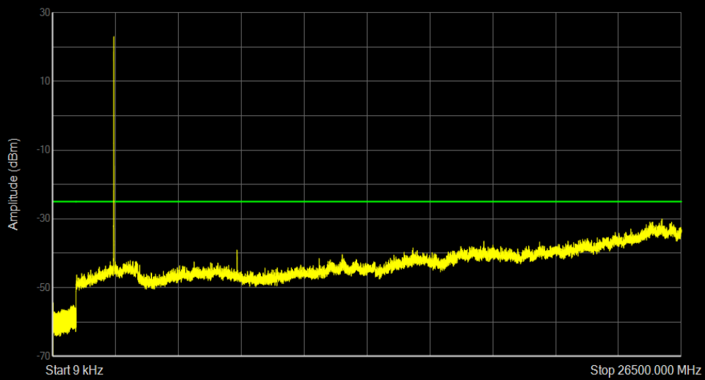
Band41(2535-2655) QAM16 BW=5MHz Channel=40640 RB Size=25 Position=#0
