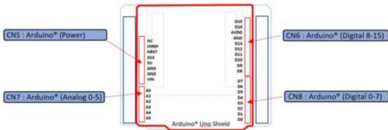
Figure 11 ARDUINO® Uno connectors and ARDUINO® shield location
