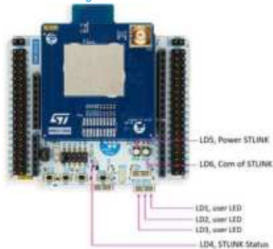
Figure 7 LEDs location
