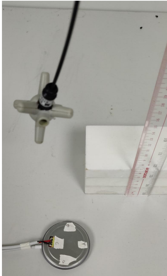
E-field Test Setup Photo of Position E(20cm)
