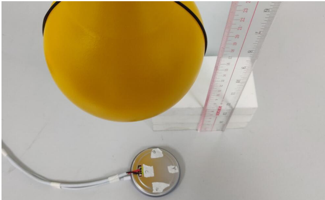
H-field Test Setup Photo of Position E(20cm)
