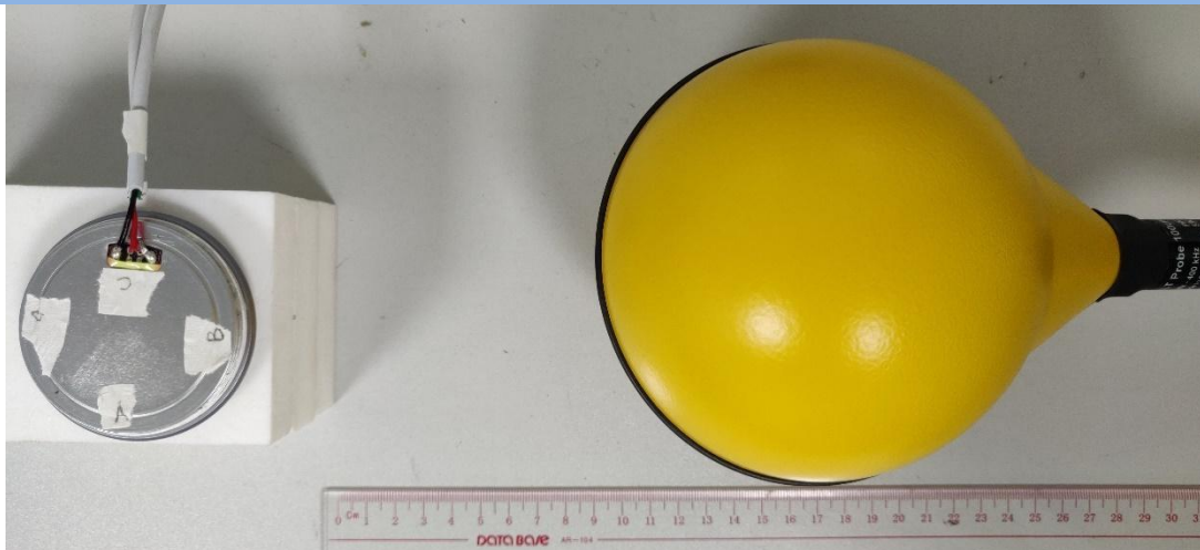
H-field Test Setup Photo of Position B(15cm)
