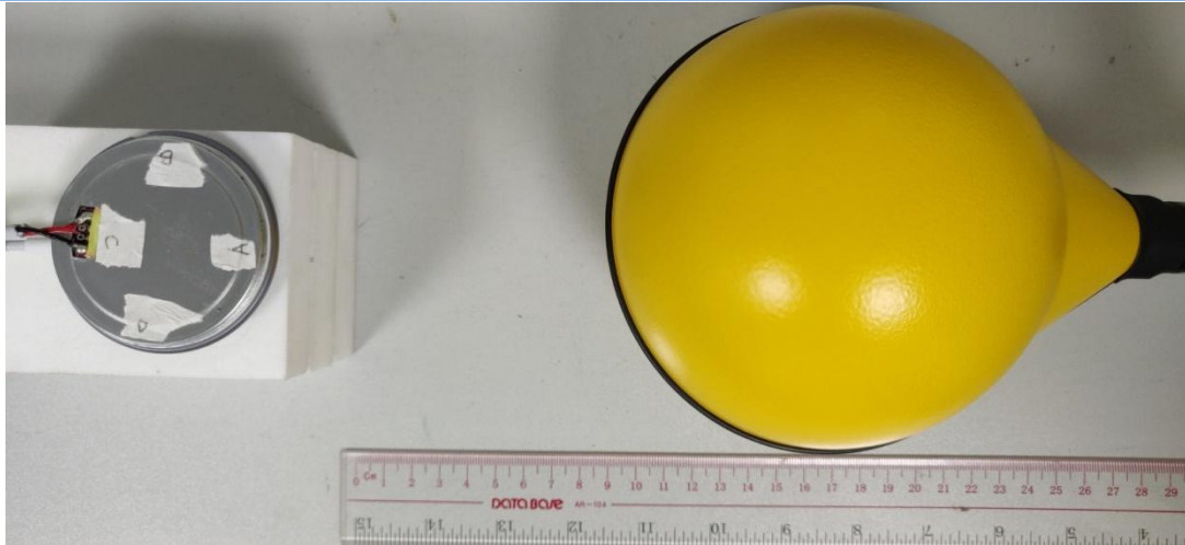
H-field Test Setup Photo of Position A(15cm)
