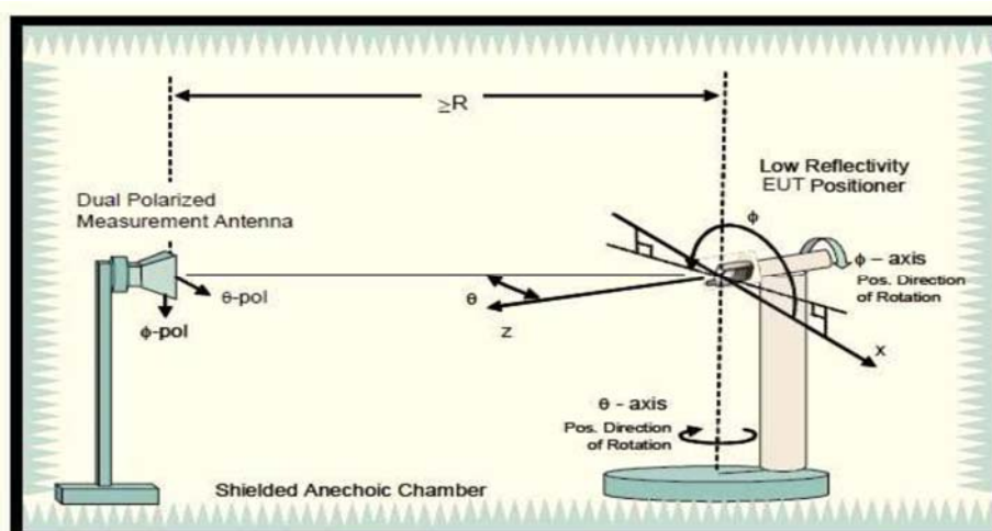
Figure 2. Configuration of Conical circle cut test system.
