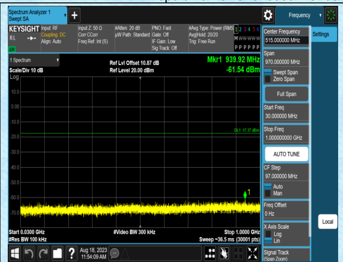
TX-Ant1-2480-30~1000
