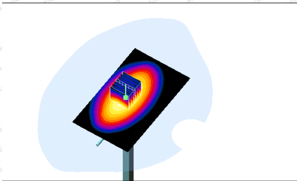
System Performance Check 835MHz Head 250mW
