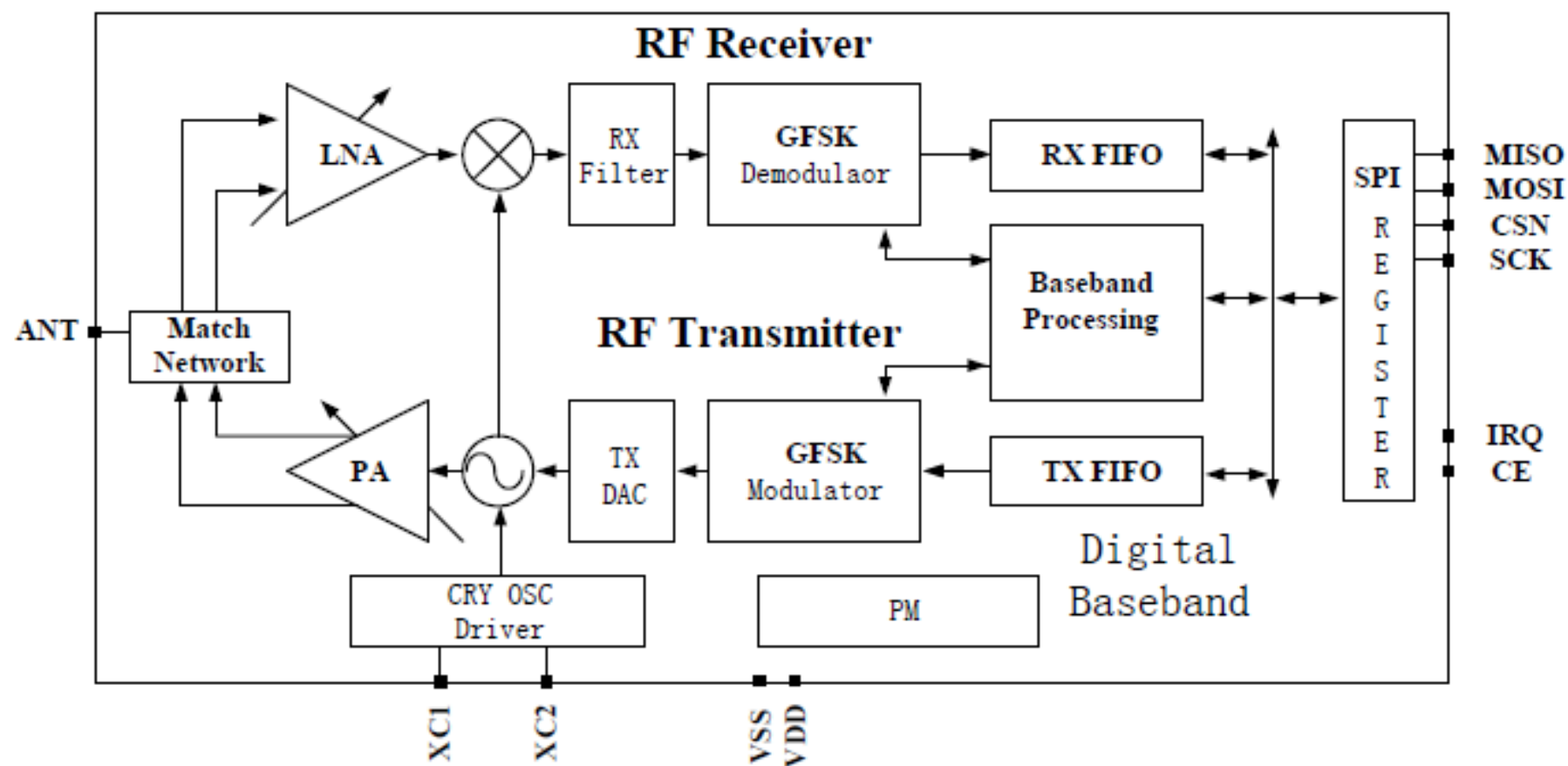
Figure 1 XN297LBW block diagram
