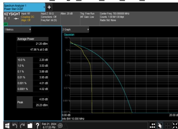
N14(10M)_DFT-s-OFDM_PI_2-BPSK_Edge_1RB_Left_Mid_CH
