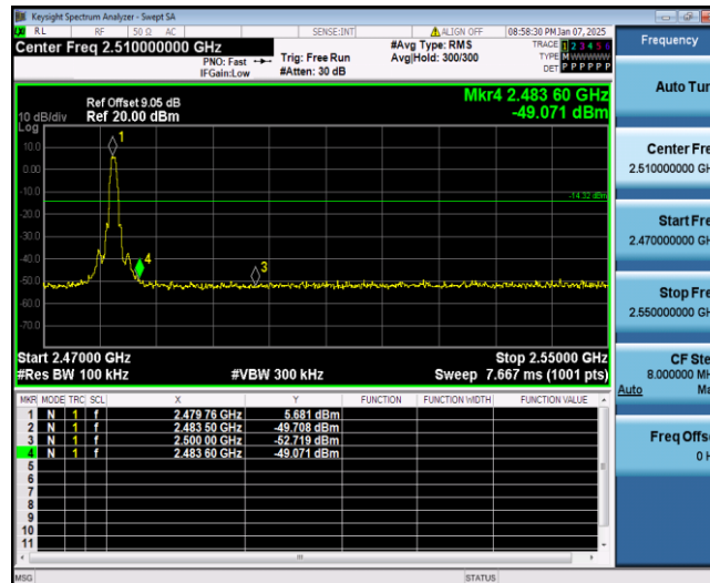
BLE_Ant1_High_2480
