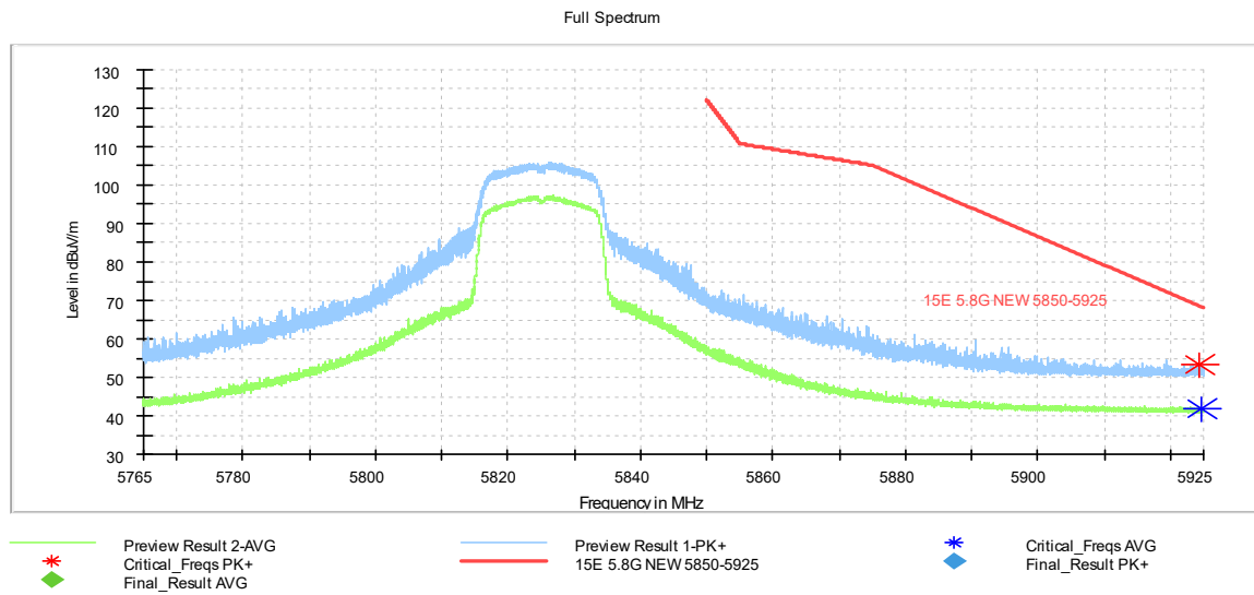
Fig. 4 Band Edges (802.11n-HT20 Ch165, 5825MHz)
