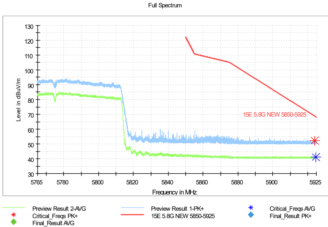
Fig. 11 Band Edges (802.11ac-HT80 Ch155, 5775MHz)
