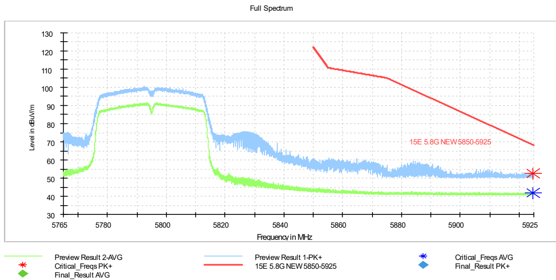
Fig. 6 Band Edges (802.11n-HT40 Ch159, 5795MHz)
