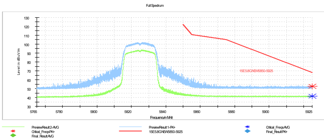
Fig. 8 Band Edges (802.11ac-HT20 Ch165, 5825MHz)
