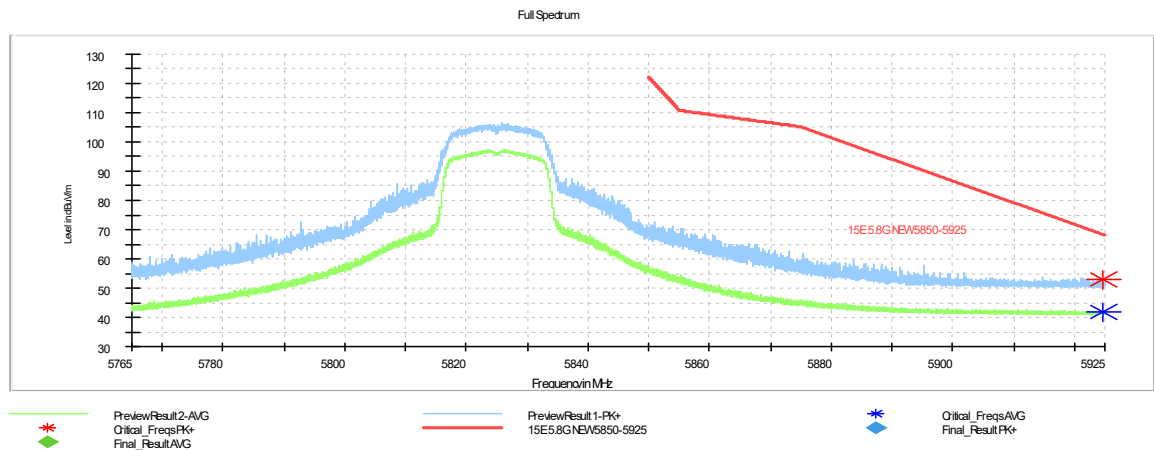
Fig. 2 Band Edges (802.11a Ch165, 5825MHz)
