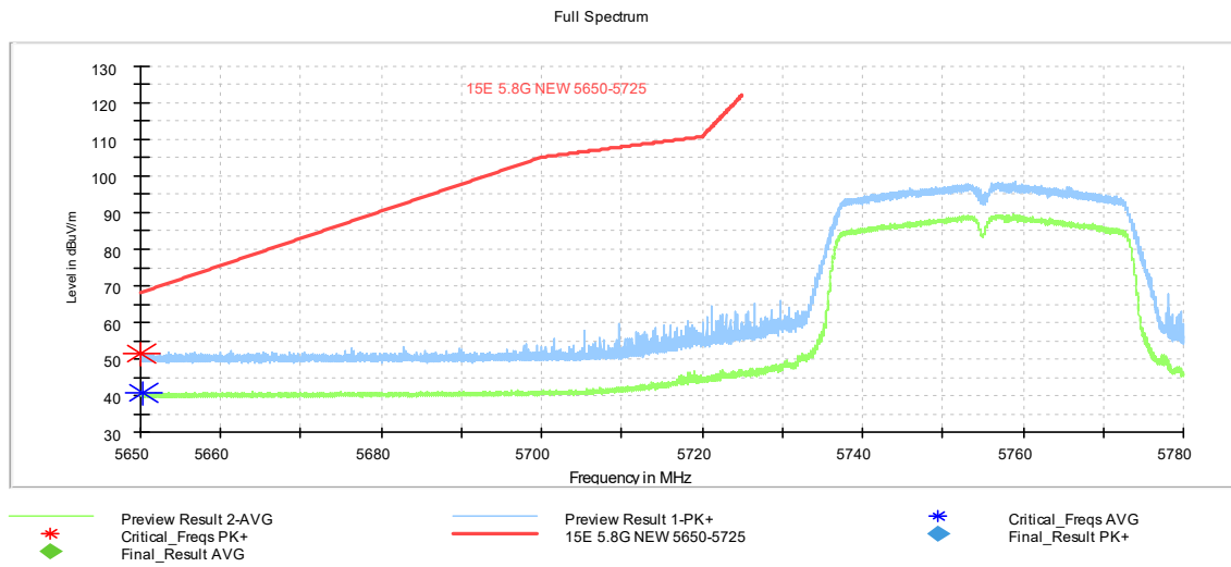
Fig. 9 Band Edges (802.11ac-HT40 Ch151, 5755MHz)
