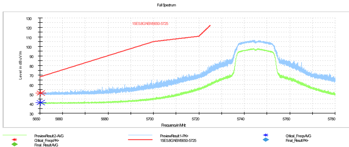
Fig. 1 Band Edges (802.11a Ch149,5745MHz)
