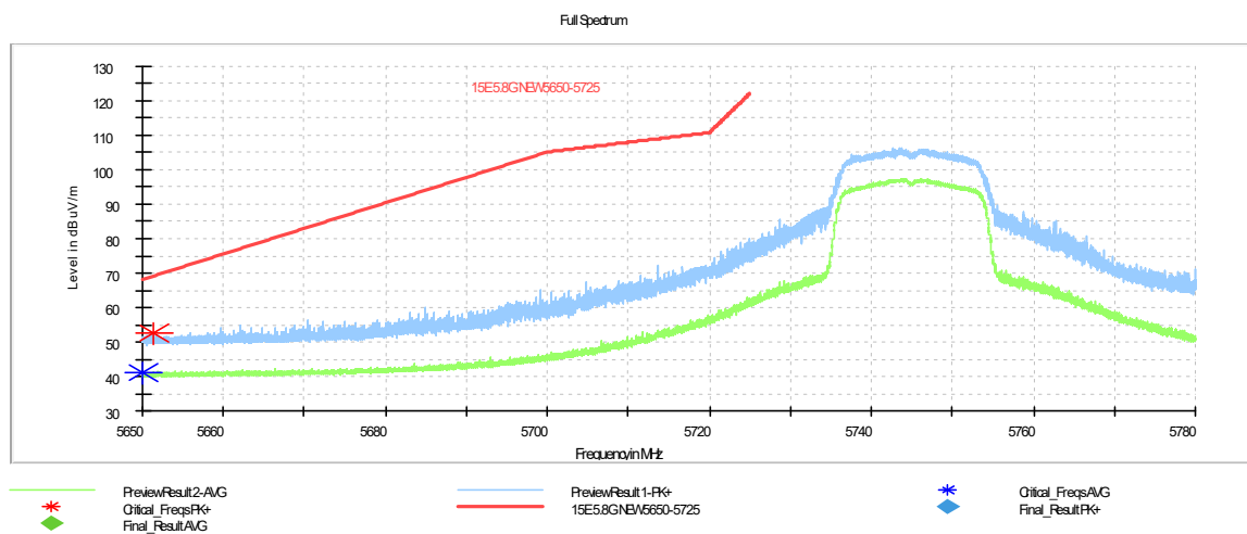
Fig. 3 Band Edges (802.11n-HT20 Ch149, 5745MHz)
