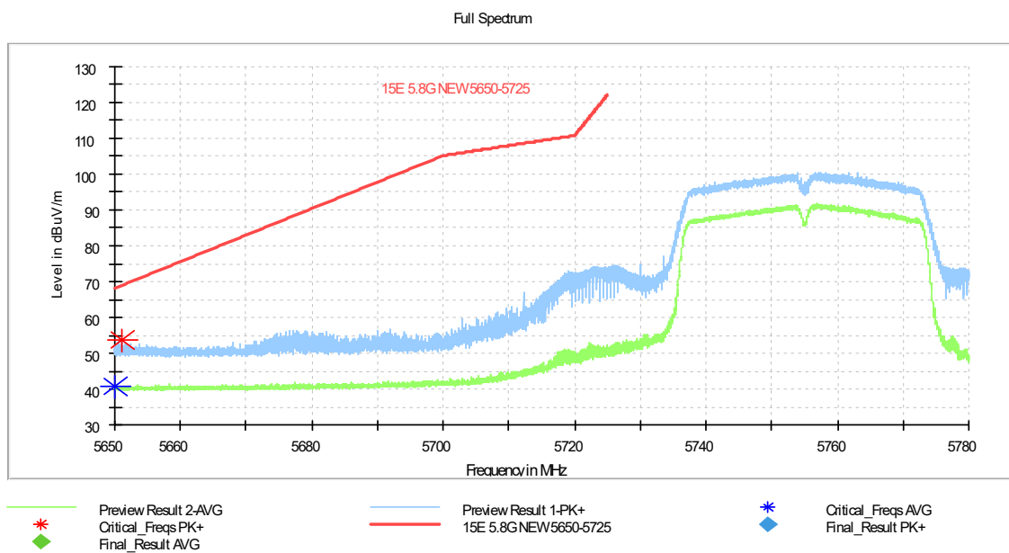
Fig. 5 Band Edges (802.11n-HT40 Ch151, 5755MHz)
