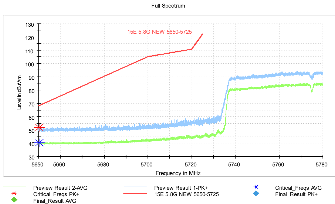
Fig. 11 Band Edges (802.11ac-HT80 Ch155, 5775MHz)
