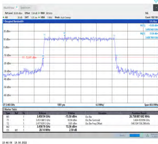
1-N78-3450-3550-PC2-30-30-L-4-DFT-64QAM-Outer_Full-75@0-Ant1-26.759-28.140-≤30-PASS
