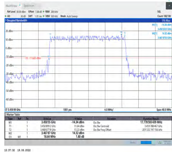
1-N78-3450-3550-PC2-30-20-L-2-DFT-PI2BPSK-Out_er_Full-50@0-Ant1-17.779-18.640-≤20-PASS
