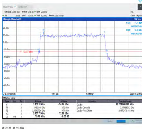
1-N78-3450-3550-PC2-30-20-L-7-CP-16QAM-Outer _Full-51@0-Ant1-18.224-19.480-≤20-PASS
