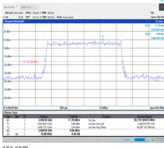
1-N78-3450-3550-PC2-30-20-L-9-CP-256QAM-Oute r_Full-51@0-Ant1-18.179-19.080-≤20-PASS
