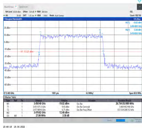
1-N78-3450-3550-PC2-30-30-L-5-DFT-256QAM-Outer_Full-75@0-Ant1-26.734-27.840-≤30-PASS
