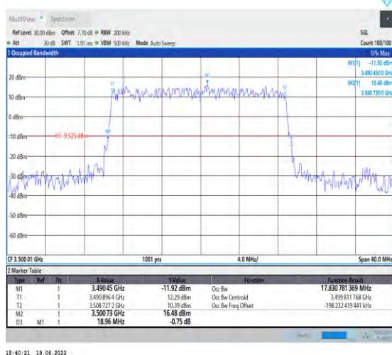
1-N78-3450-3550-PC2-30-20-M-2-DFT-PI2BPSK-Outer _Full-50@0-Ant1-17.831-18.960-≤20-PASS
