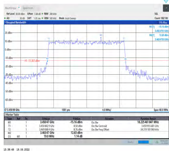
1-N78-3450-3550-PC2-30-20-L-8-CP-64QAM-Outer _Full-51@0-Ant1-18.225-19.000-≤20-PASS
