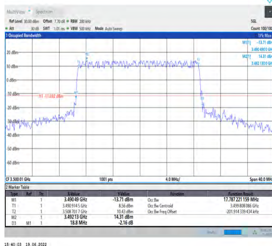
1-N78-3450-3550-PC2-30-20-M-1-DFT-QPSK-Outer _Full-50@0-Ant1-17.787-18.800-≤20-PASS
