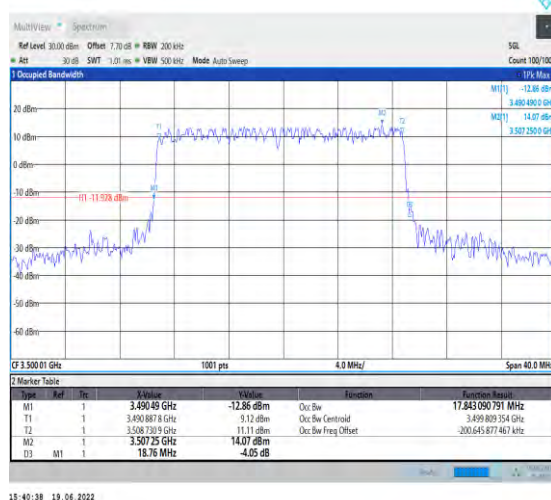
1-N78-3450-3550-PC2-30-20-M-3-DFT-16QAM-Outer _Full-50@0-Ant1-17.843-18.760-≤20-PASS
