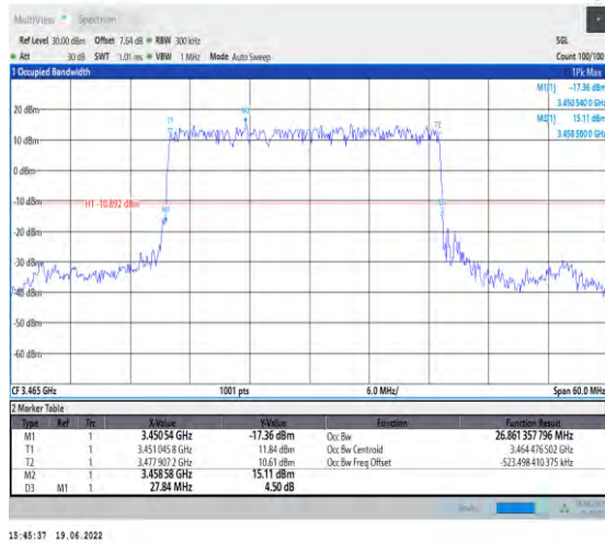
1-N78-3450-3550-PC2-30-30-L-2-DFT-PI2BPSK-Out er_Full-75@0-Ant1-26.861-27.840-≤30-PASS
