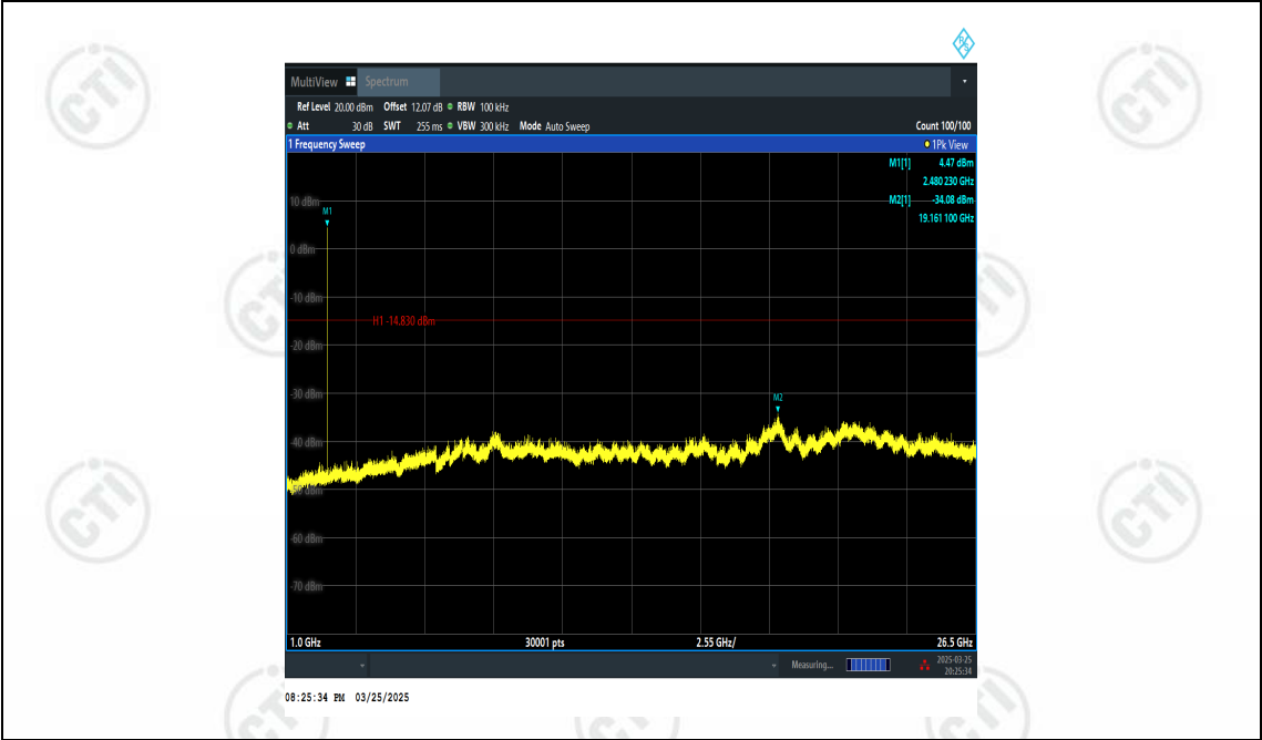
DH5-Ant1-2480-1000~26500-PASS
