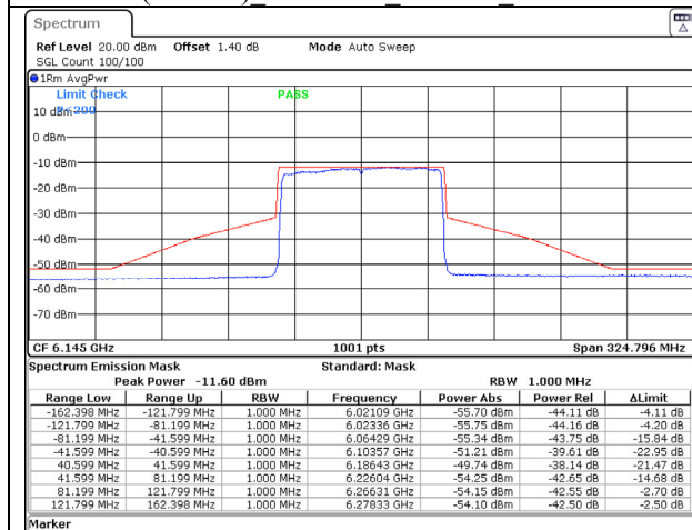
802.11ax (80MHz) 6145MHz Chain A NSS-1
