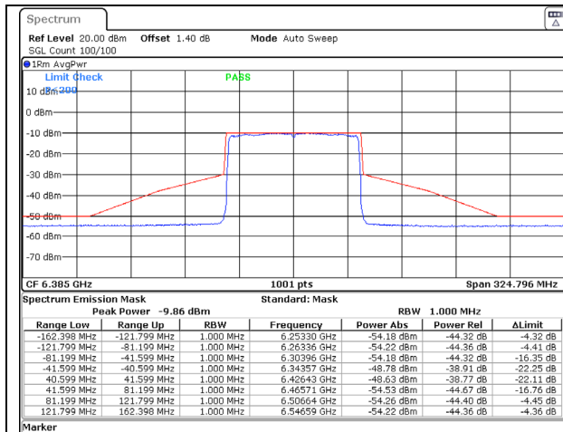
802.11ax (80MHz) 6385MHz Chain C NSS-1
