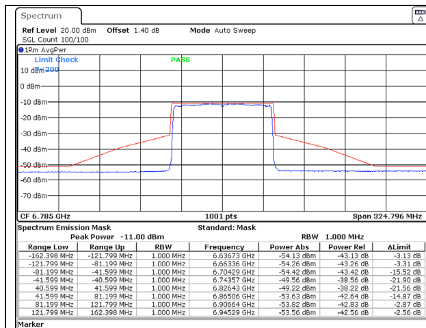
802.11ax (80MHz) 6785MHz Chain A NSS-1
