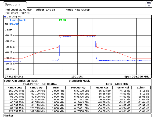
802.11ax (80MHz) 6145MHz Chain D NSS-1
