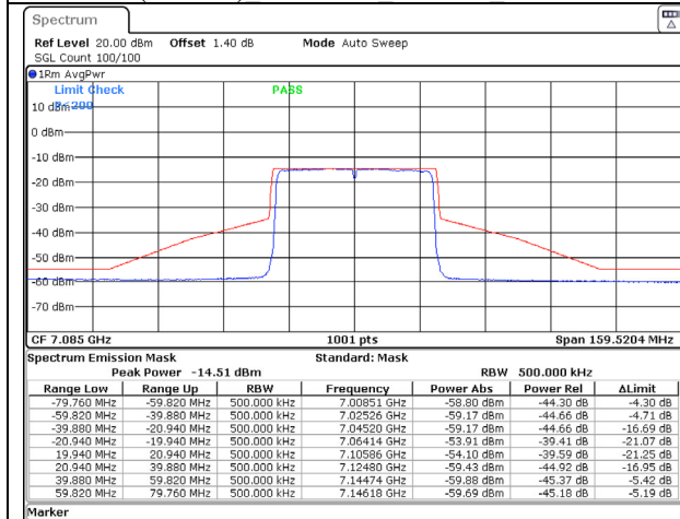
802.11ax (40MHz) 7085MHz Chain A NSS-1
