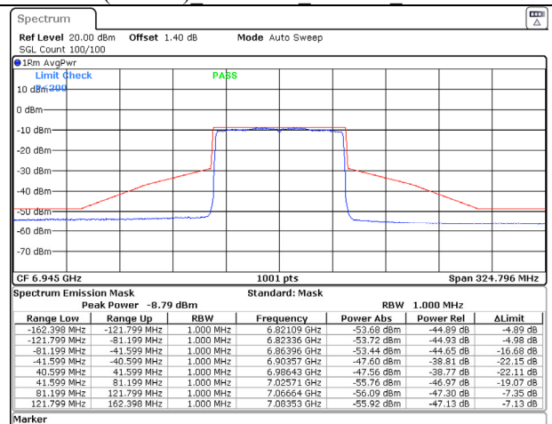
802.11ax (80MHz) 6945MHz Chain B NSS-1
