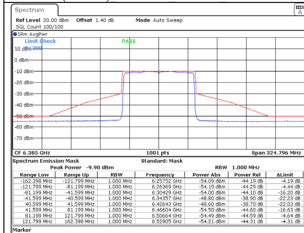
802.11ax (80MHz) 6385MHz Chain A NSS-1
