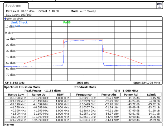
802.11ax (80MHz) 6145MHz Chain B NSS-1
