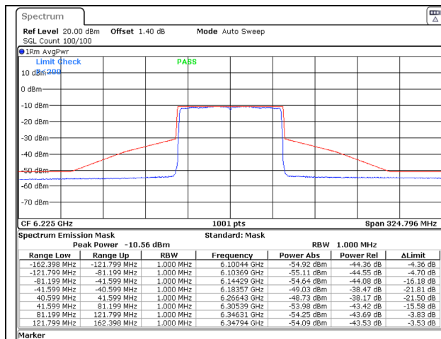
802.11ax (80MHz) 6225MHz Chain A NSS-1
