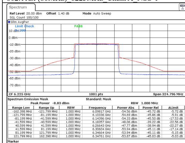
802.11ax (80MHz) 6225MHz Chain C NSS-1
