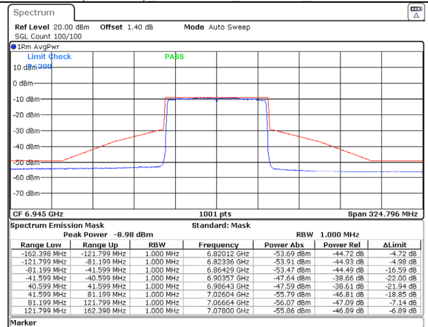
802.11ax (80MHz) 6945MHz Chain D NSS-1
