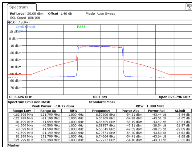
802.11ax (80MHz) 6625MHz Chain C NSS-1
