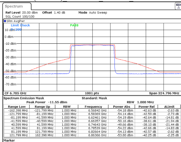
802.11ax (80MHz) 6705MHz Chain A NSS-1
