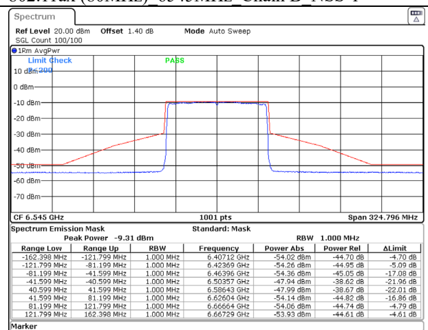
802.11ax (80MHz) 6545MHz Chain D NSS-1
