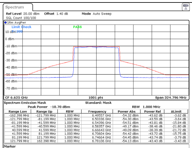
802.11ax (80MHz) 6625MHz Chain D NSS-1
