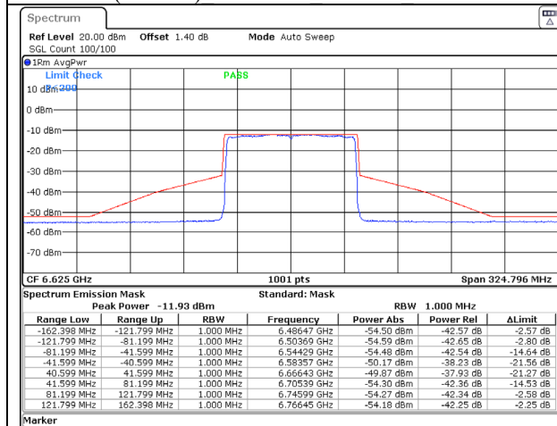
802.11ax (80MHz) 6625MHz Chain A NSS-1
