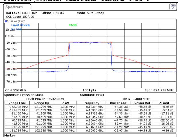
802.11ax (80MHz) 6225MHz Chain D NSS-1
