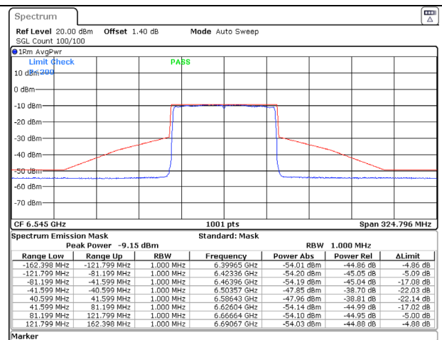
802.11ax (80MHz) 6545MHz Chain B NSS-1
