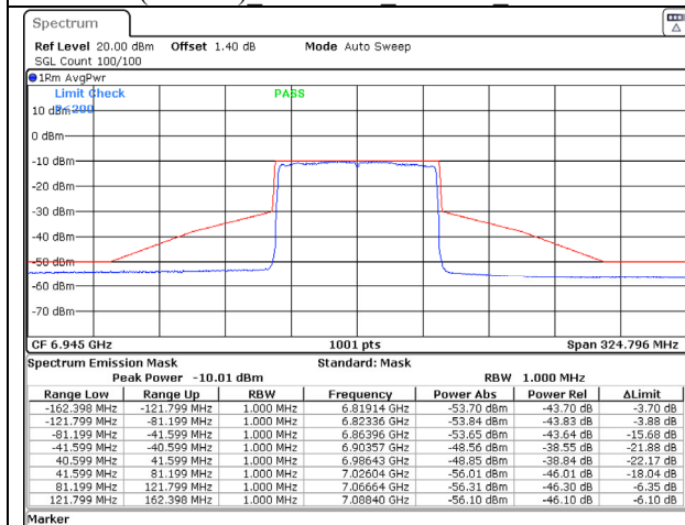
802.11ax (80MHz) 6945MHz Chain A NSS-1
