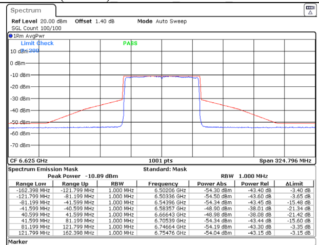
802.11ax (80MHz) 6625MHz Chain B NSS-1
