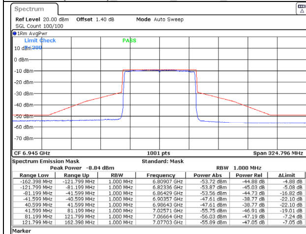
802.11ax (80MHz) 6945MHz Chain C NSS-1
