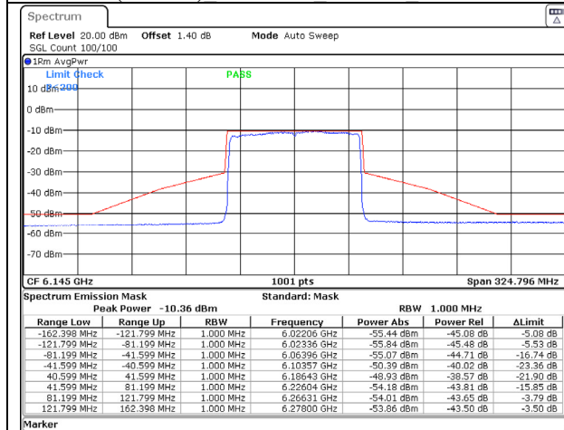
802.11ax (80MHz) 6145MHz Chain C NSS-1
