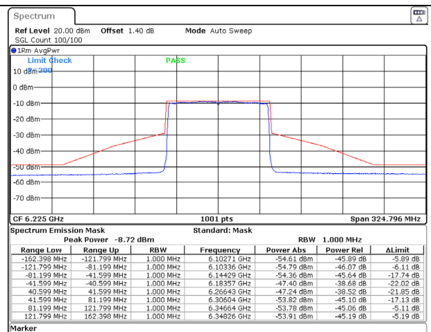
802.11ax (80MHz) 6225MHz Chain B NSS-1
