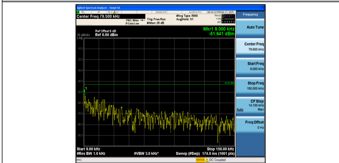
Band66_3MHz_QPSK_132322_1RB#0_0.009~0.15_0.009~0.15
