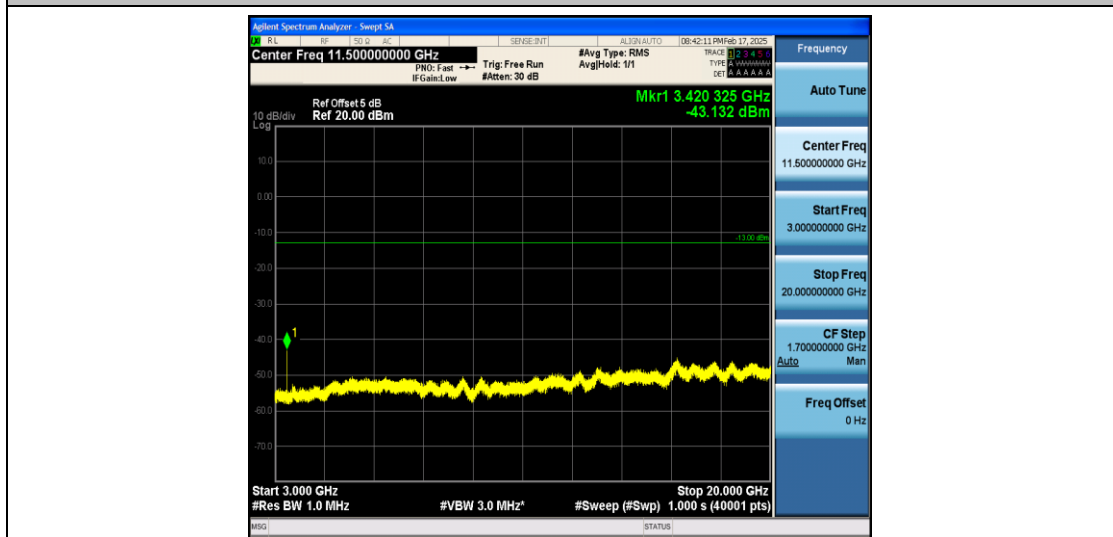
Band66_3MHz_16QAM_131987_1RB#0_3000~131022_3000~131022
