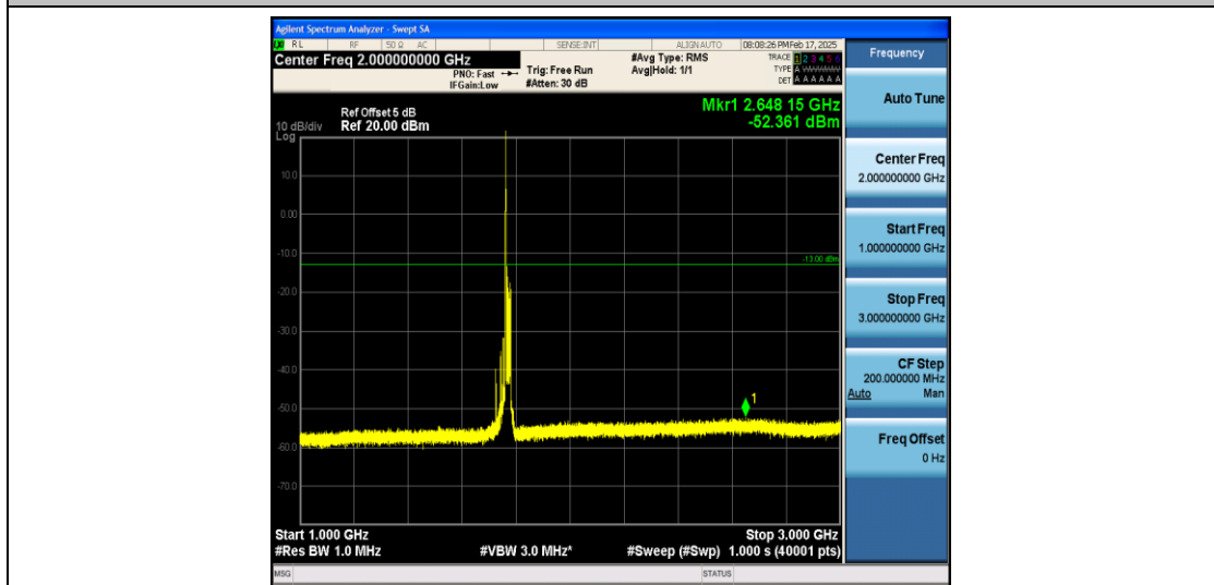
Band66_20MHz_QPSK_132572_1RB#0_1000~3000_1000~3000
