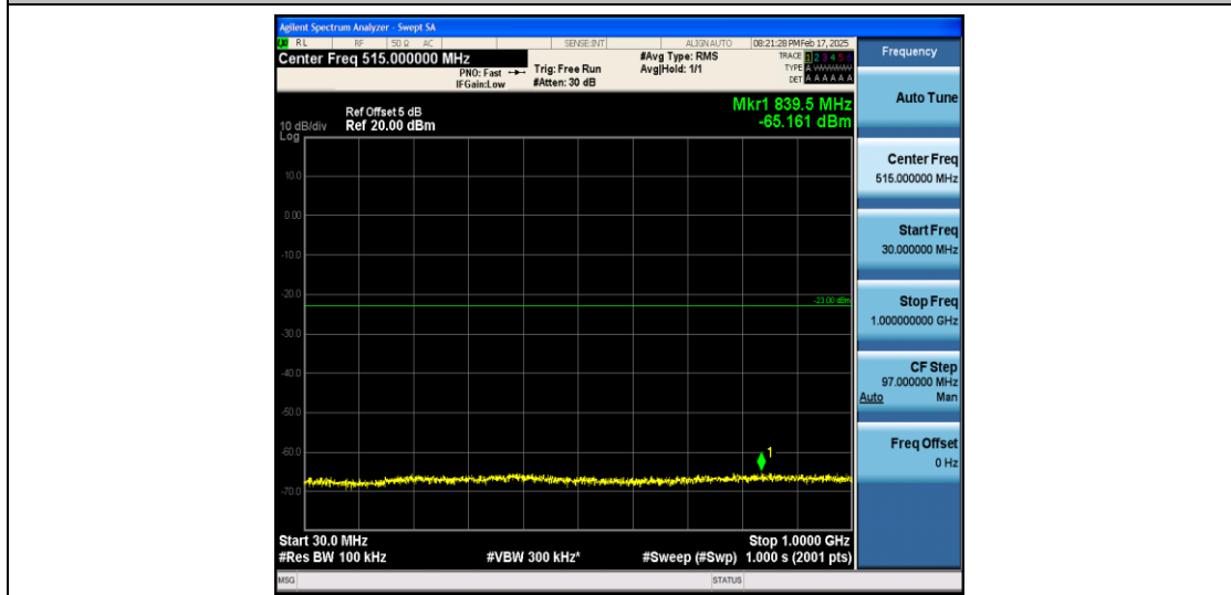
Band66_1.4MHz_QPSK_131979_1RB#0_30~1000_30~1000
