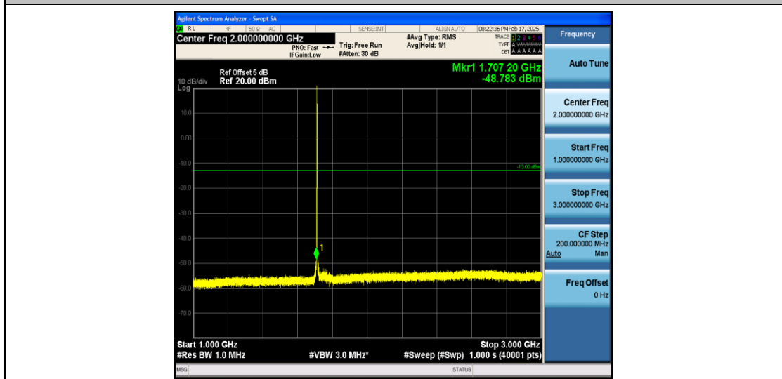
Band66_1.4MHz_16QAM_131979_1RB#0_1000~3000_1000~3000
