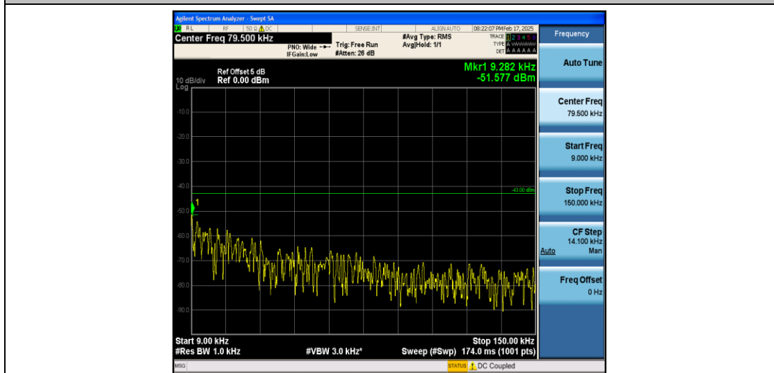
Band66_1.4MHz_16QAM_131979_1RB#0_0.009~0.15_0.009~0.15
