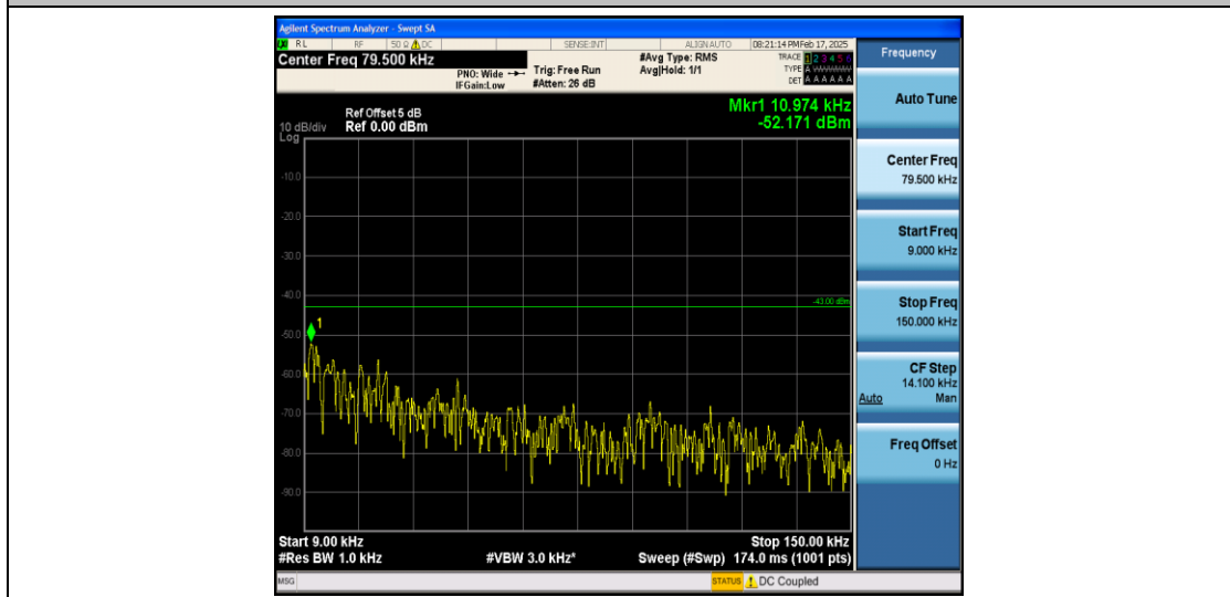
Band66_1.4MHz_QPSK_131979_1RB#0_0.009~0.15_0.009~0.15
