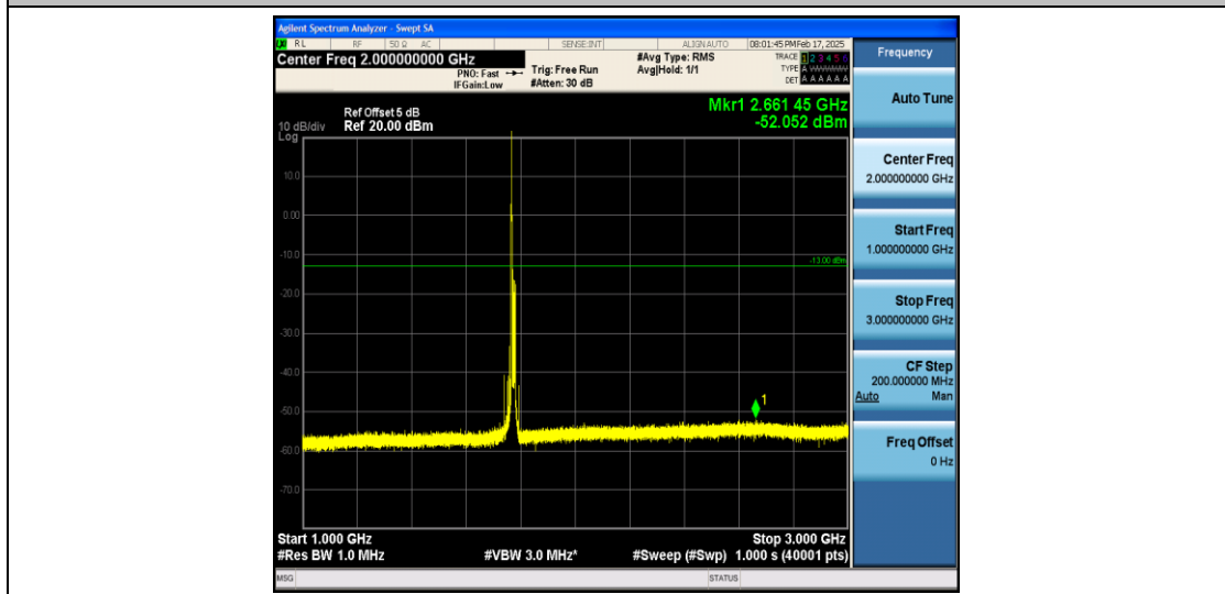
Band66_15MHz_16QAM_132597_1RB#0_1000~3000_1000~3000
