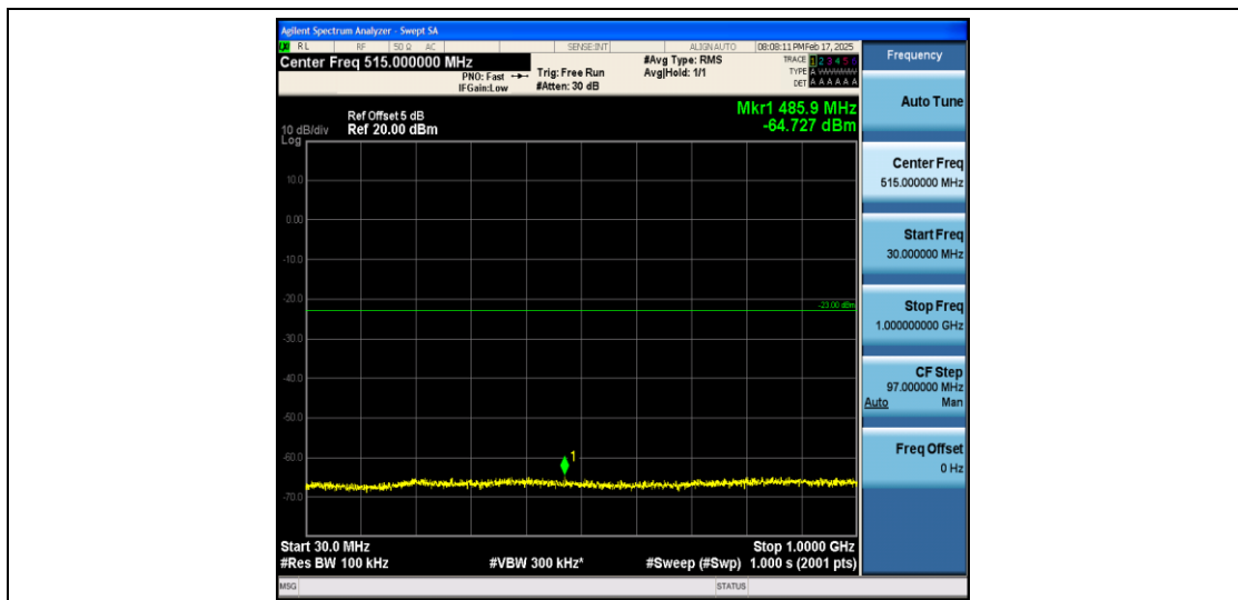
Band66_20MHz_QPSK_132572_1RB#0_30~1000_30~1000
