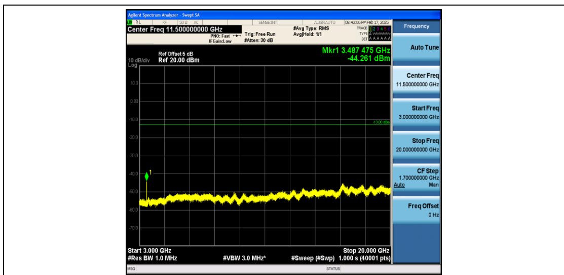
Band66_3MHz_QPSK_132322_1RB#0_3000~131022_3000~131022
