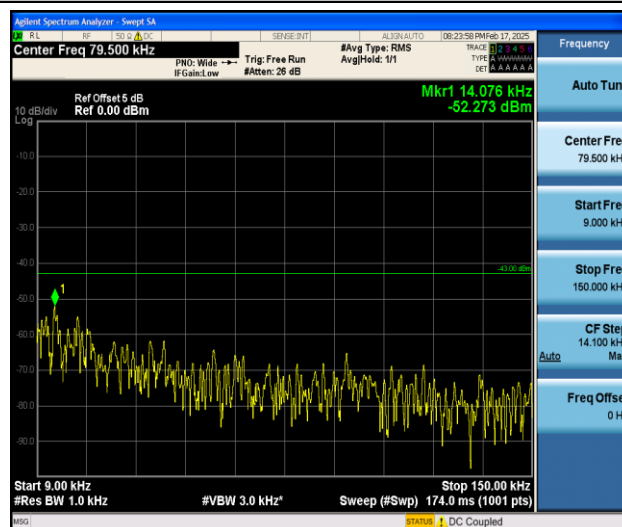
Band66_1.4MHz_16QAM_132322_1RB#0_0.009~0.15_0.009~0.15
