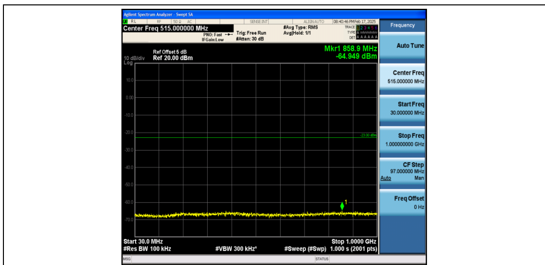
Band66_3MHz_QPSK_131987_1RB#0_30~1000_30~1000
