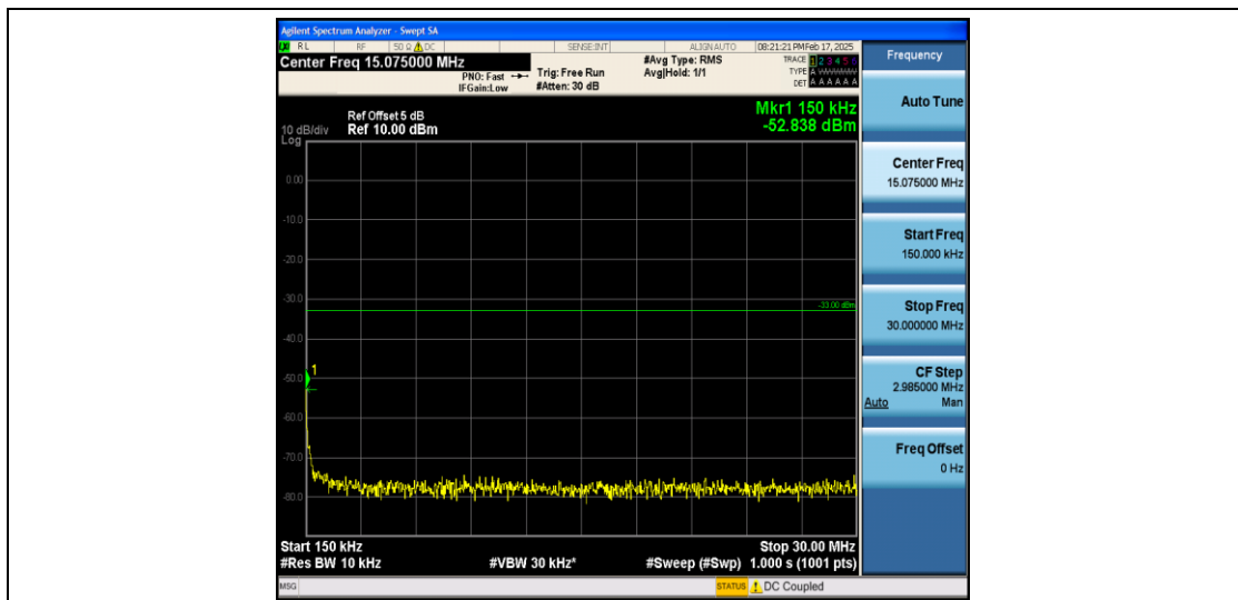
Band66_1.4MHz_QPSK_131979_1RB#0_0.15~30_0.15~30
