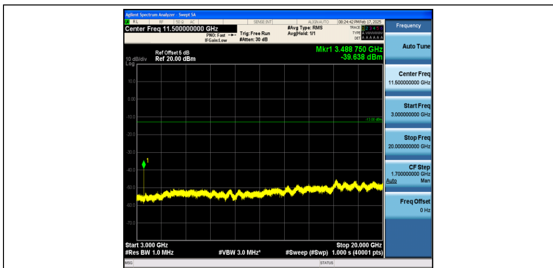
Band66_1.4MHz_16QAM_132322_1RB#0_3000~131022_3000~131022
