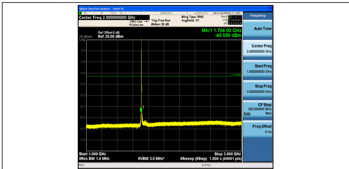
Band66_3MHz_16QAM_131987_1RB#0_1000~3000_1000~3000
