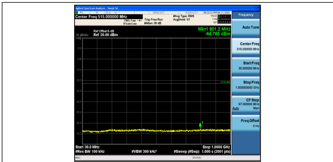
Band66_1.4MHz_16QAM_131979_1RB#0_30~1000_30~1000
