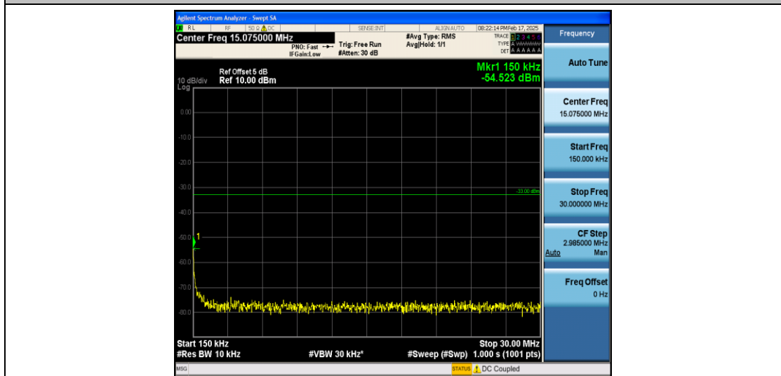
Band66_1.4MHz_16QAM_131979_1RB#0_0.15~30_0.15~30
