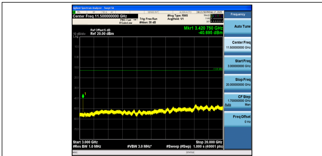
Band66_1.4MHz_QPSK_131979_1RB#0_3000~131022_3000~131022
