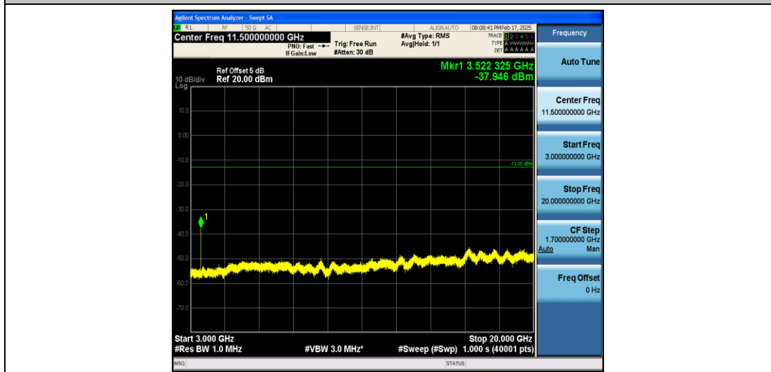
Band66_20MHz_QPSK_132572_1RB#0_3000~131022_3000~131022
