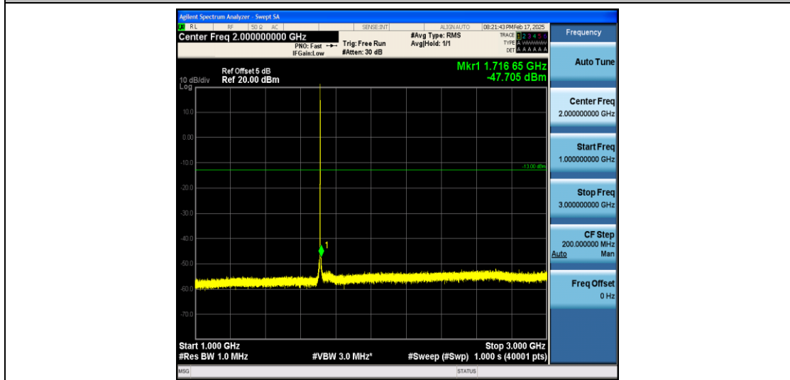
Band66_1.4MHz_QPSK_131979_1RB#0_1000~3000_1000~3000
