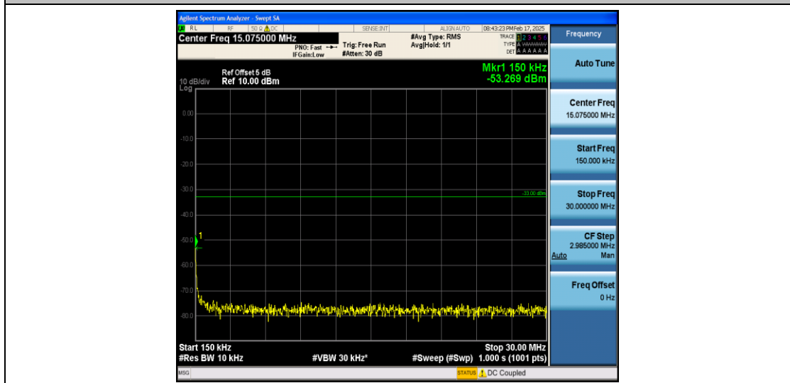
Band66_3MHz_16QAM_132322_1RB#0_0.15~30_0.15~30
