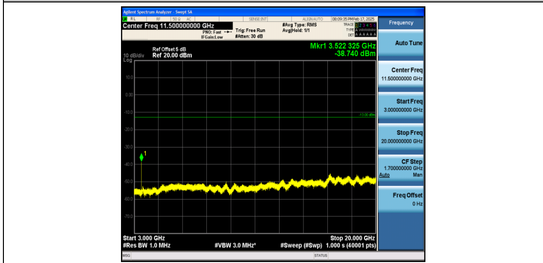
Band66_20MHz_16QAM_132572_1RB#0_3000~131022_3000~131022
