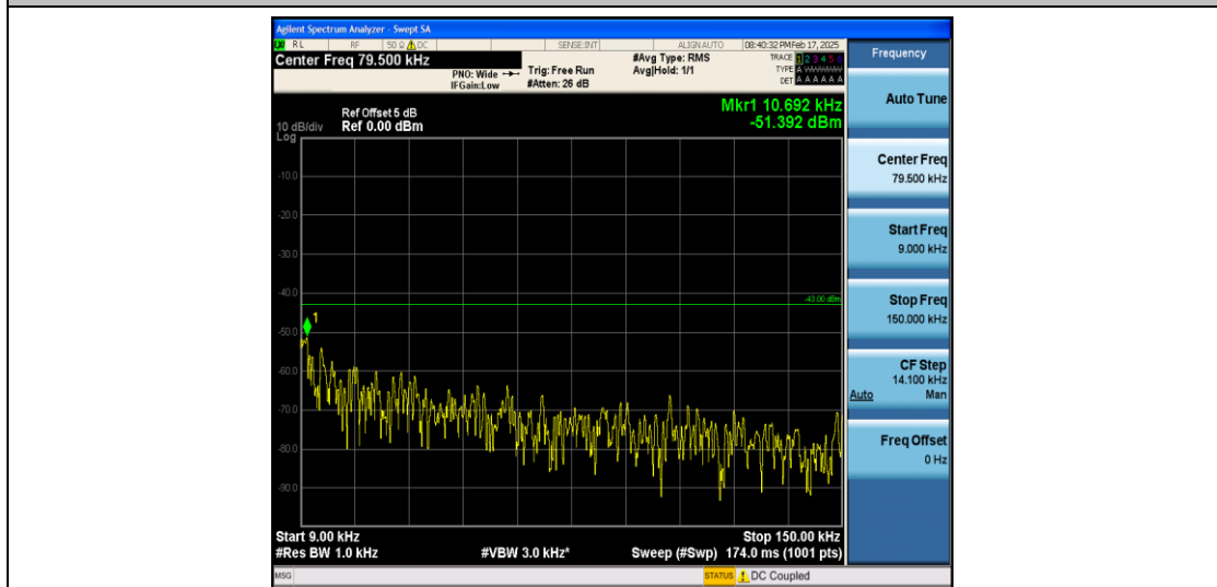
Band66_3MHz_QPSK_131987_1RB#0_0.009~0.15_0.009~0.15
