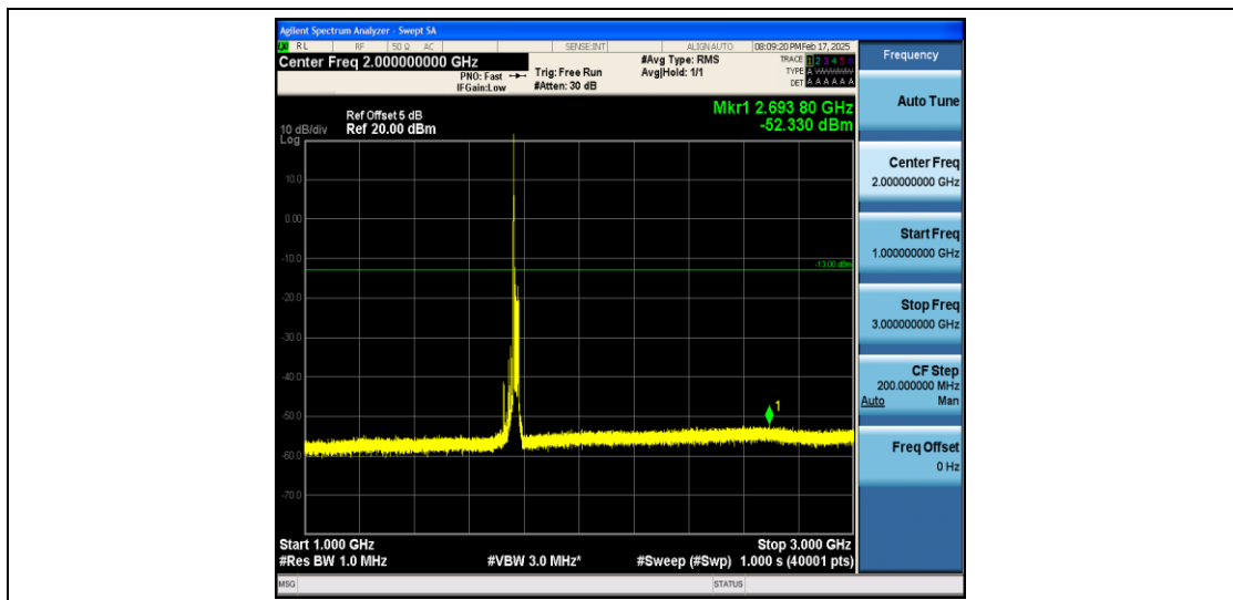
Band66_20MHz_16QAM_132572_1RB#0_1000~3000_1000~3000
