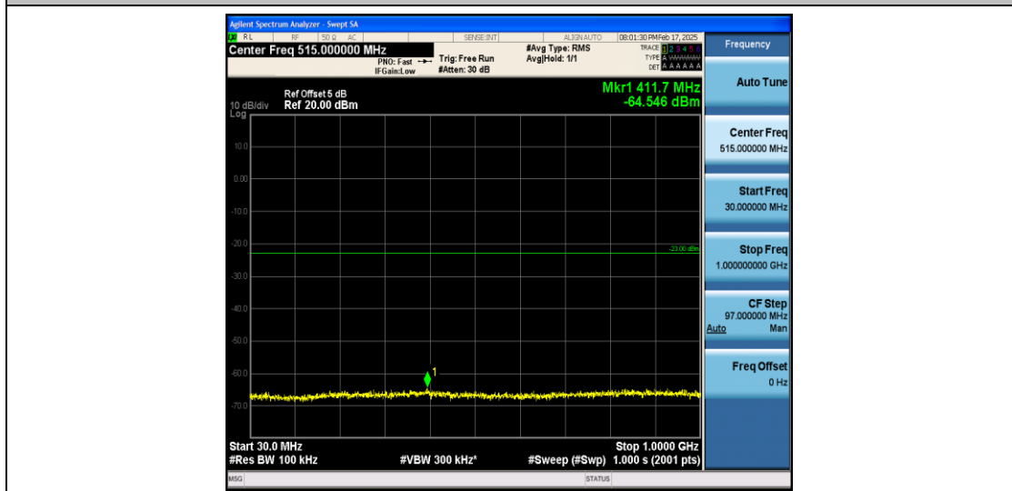
Band66_15MHz_16QAM_132597_1RB#0_30~1000_30~1000
