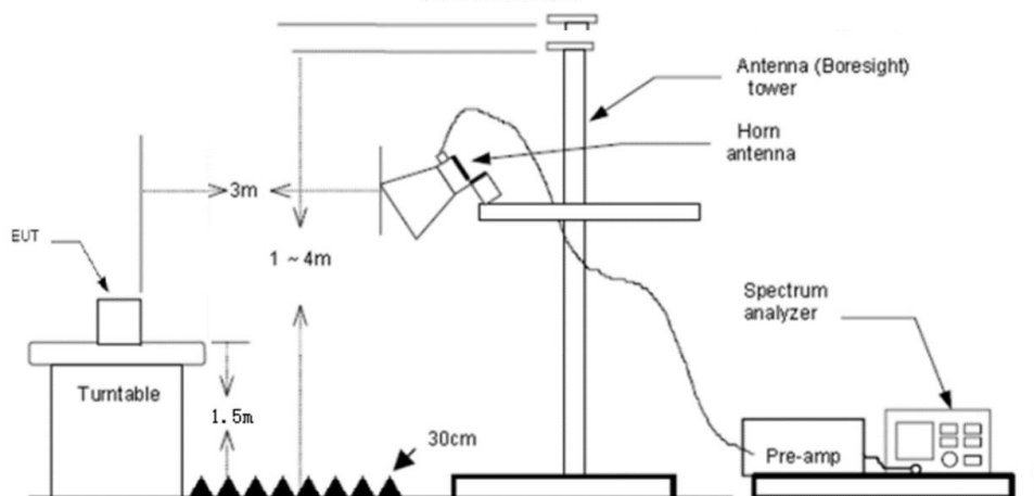
Above 1GHz
