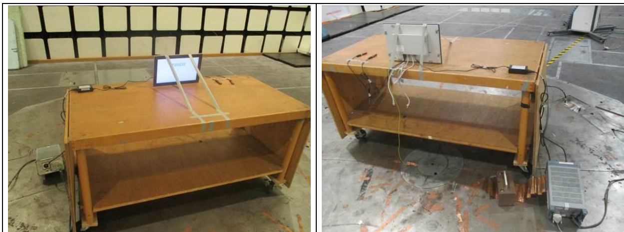
Figure 6-1: test setup Low voltage AC mains continuous disturbance
