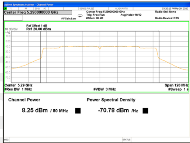
5290MHz_AV_Ant A
