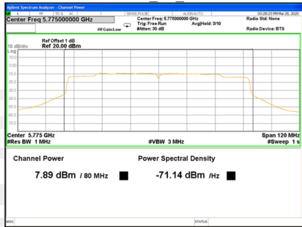
5775MHz_AV_Ant B
