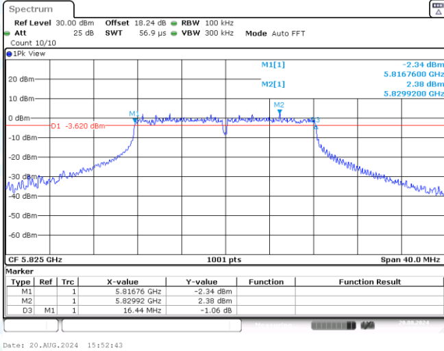
11A-Ant3-5825-PASS
