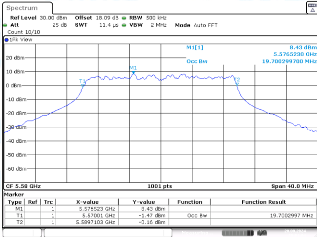
11AX20ISO-Ant3-5580
