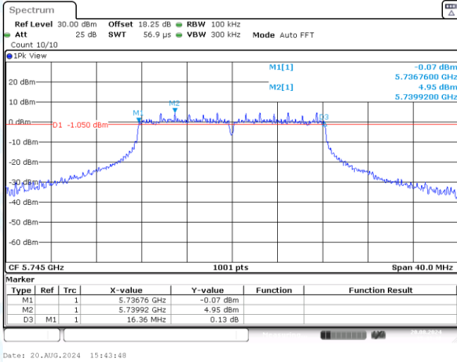
11A-Ant3-5745-PASS
