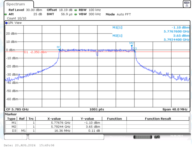
11A-Ant3-5785-PASS
