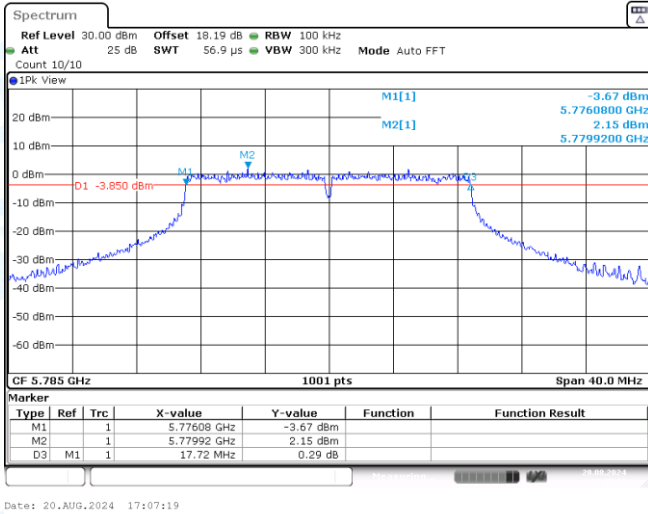
11N20SISO-Ant3-5785-PASS
