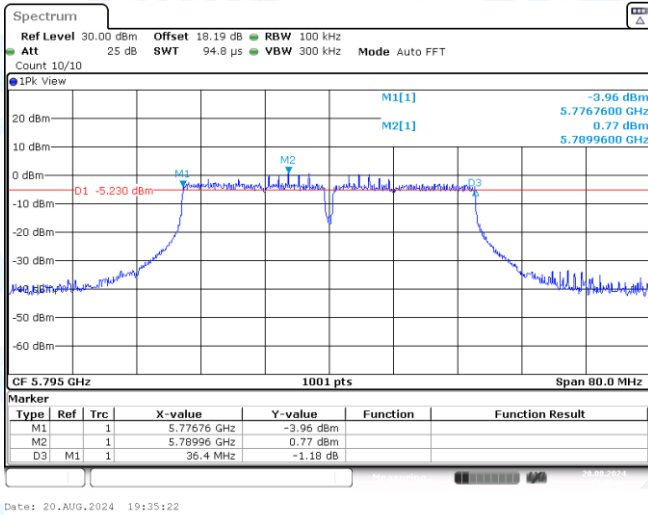
11AC40SISO-Ant3-5795-PASS
