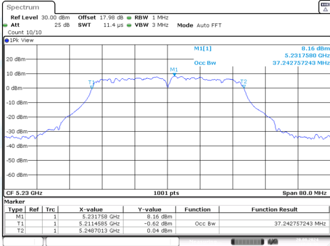
11N40SISO-Ant3-5230
