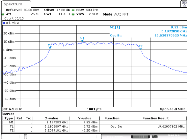
11AX20SISO-Ant3-5200
