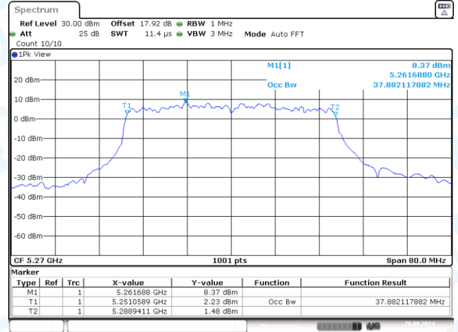
11AX40SISO-Ant3-5270
