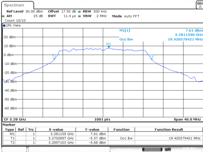
11AC20SISO-Ant3-5280
