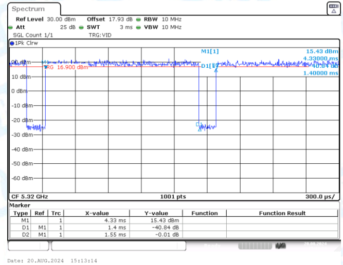
NTNV-11A-Ant3-5320
