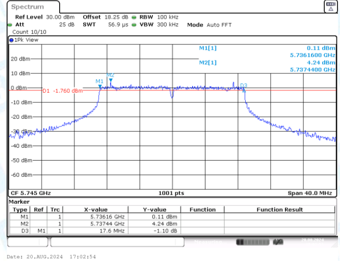
11N20SISO-Ant3-5745-PASS
