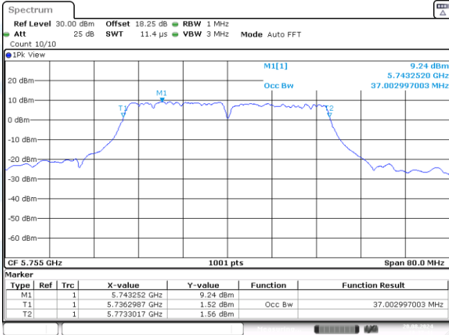
11N40SISO-Ant3-5755
