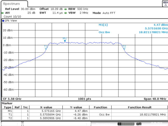
11N20SISO-Ant3-5580
