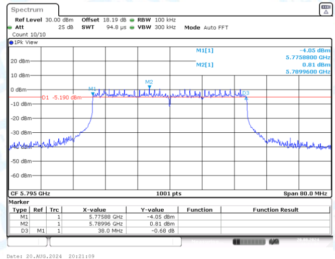
11AX40SISO-Ant3-5795-PASS
