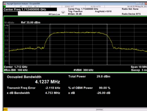
(Plot G1: WCDMA 1700MHz Channel = 1312 bandwidth)
