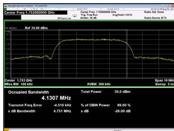
(Plot G2: WCDMA 1700 MHz Channel = 1513 bandwidth)
