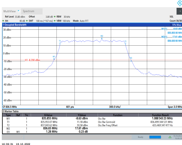
Band26-1.4MHz-QPSK-26915-6RB#0
