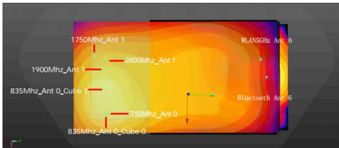
WWAN+WLAN+BT_Body worn_Back_5mm
