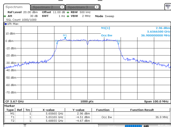
n40_5670MHz_Chain 0
