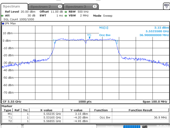
n40_5550MHz_Chain 0
