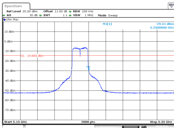
n20_5240MHz_Chain 0
