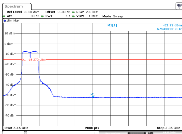
n20_5180MHz_Chain 0
