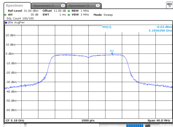
n20_5180MHz_Chain 0
