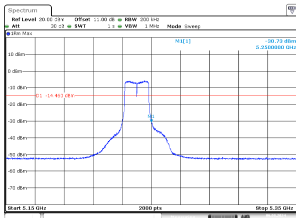
a_5240MHz_Chain 0
