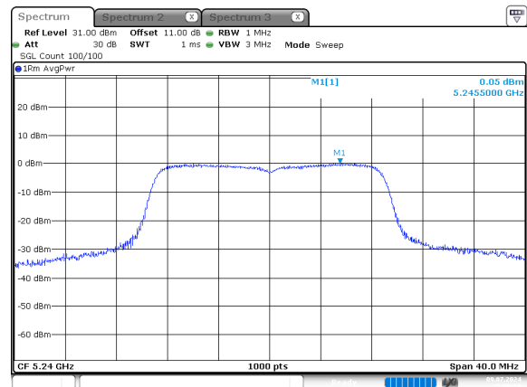
n20_5240MHz_Chain 0
