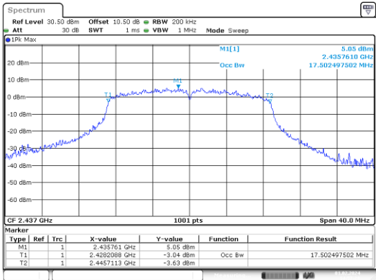
n20_2437MHz
