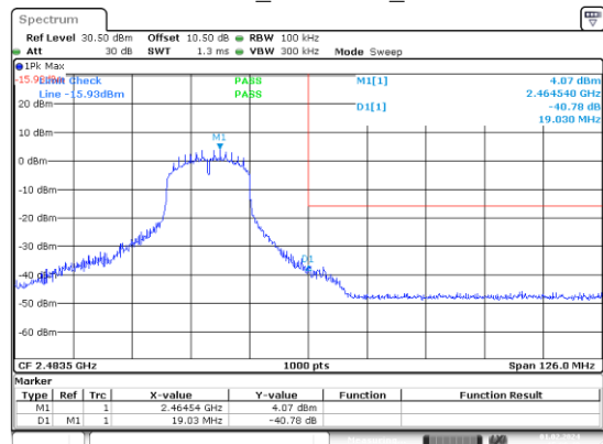
n20_2462MHz_
