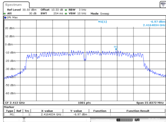
g_2412MHz
