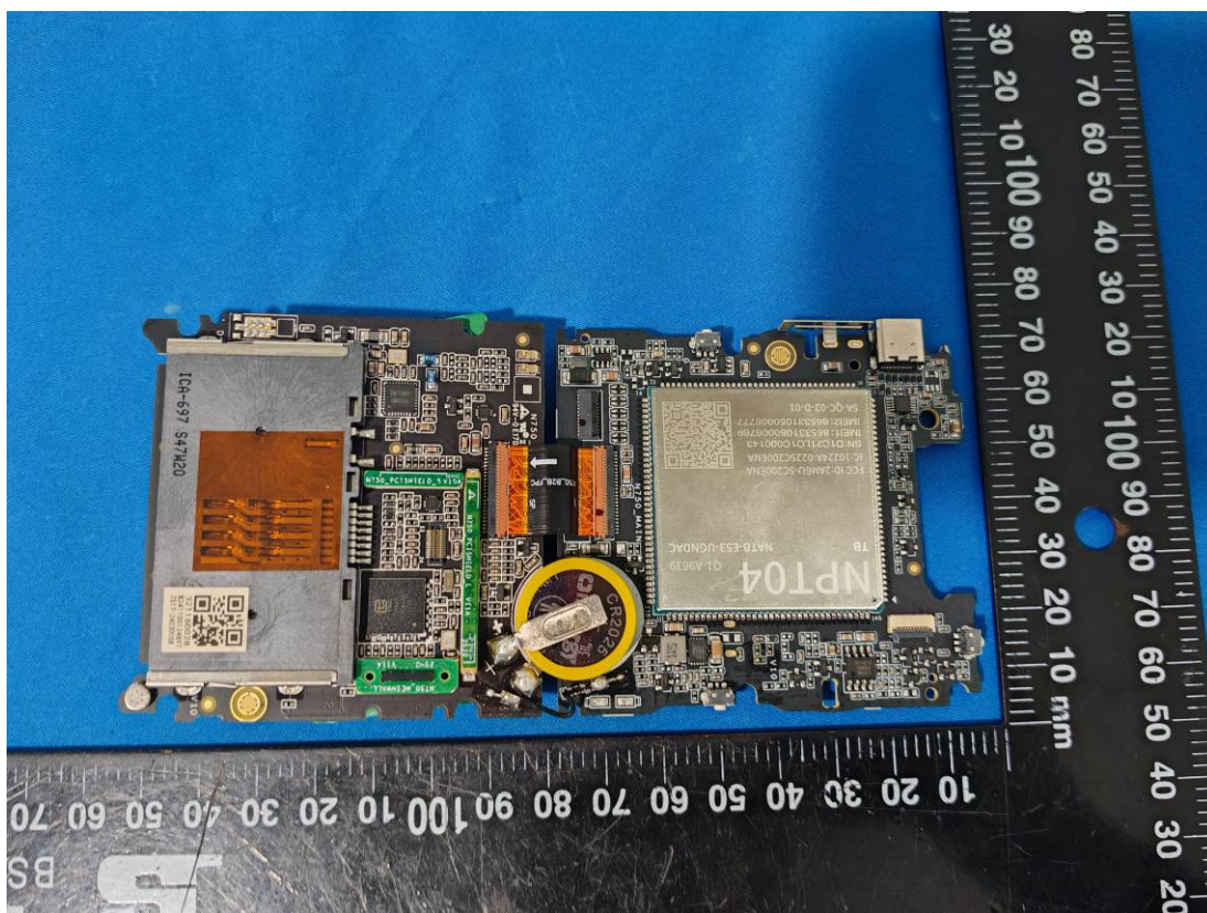
Fixture board
