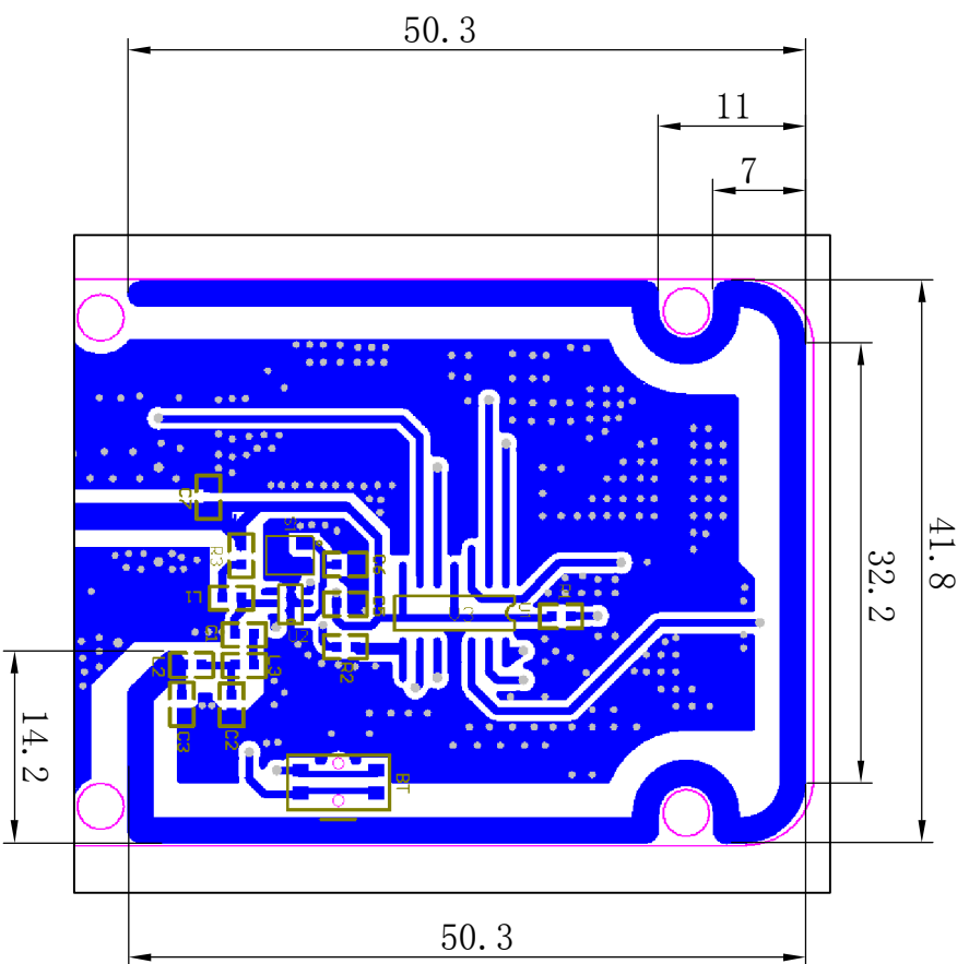
GG2017-17T4 Schematic diagram of antenna position
