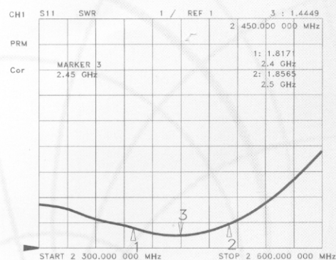
SWR
