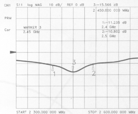
Return Loss
