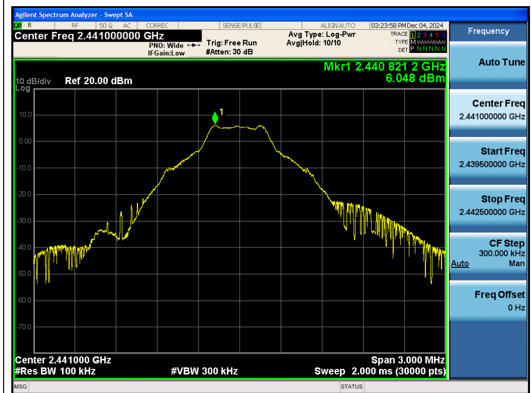
Test_Graph_BR_ANT1_2441_1Mbps_Reference Level
