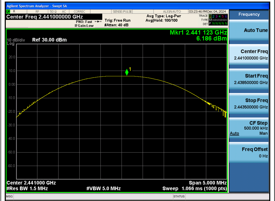
Test_Graph_BR_ANT1_2441_1Mbps_Peak Power
