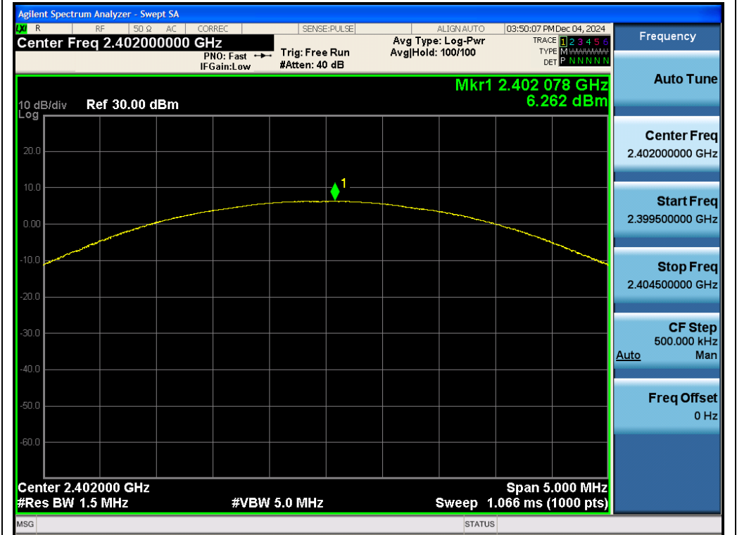
Test_Graph_EDR_ANT1_2402_2Mbps_Peak Power
