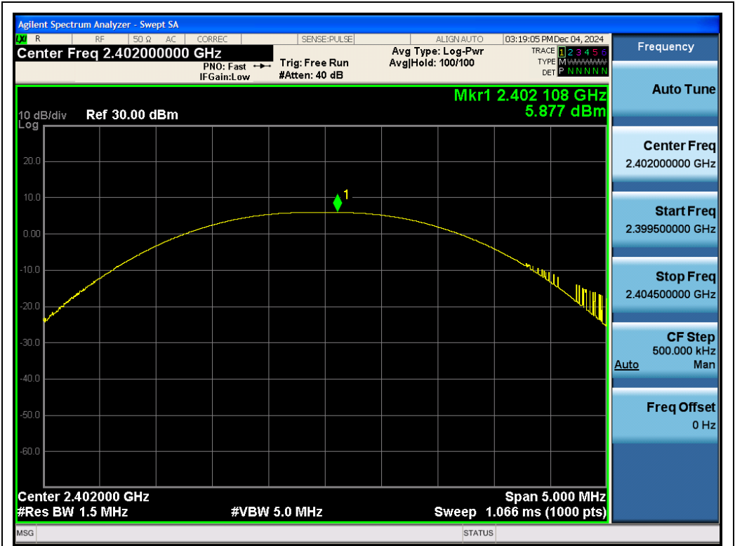
Test_Graph_BR_ANT1_2402_1Mbps_Peak Power
