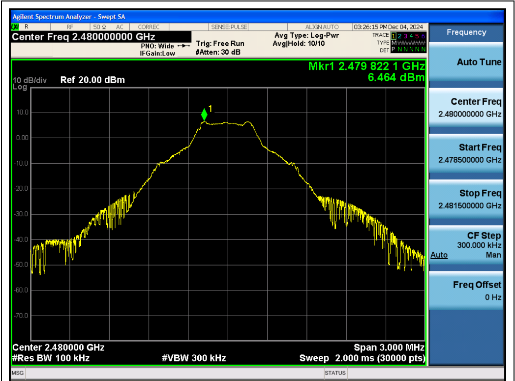
Test_Graph_BR_ANT1_2480_1Mbps_Reference Level
