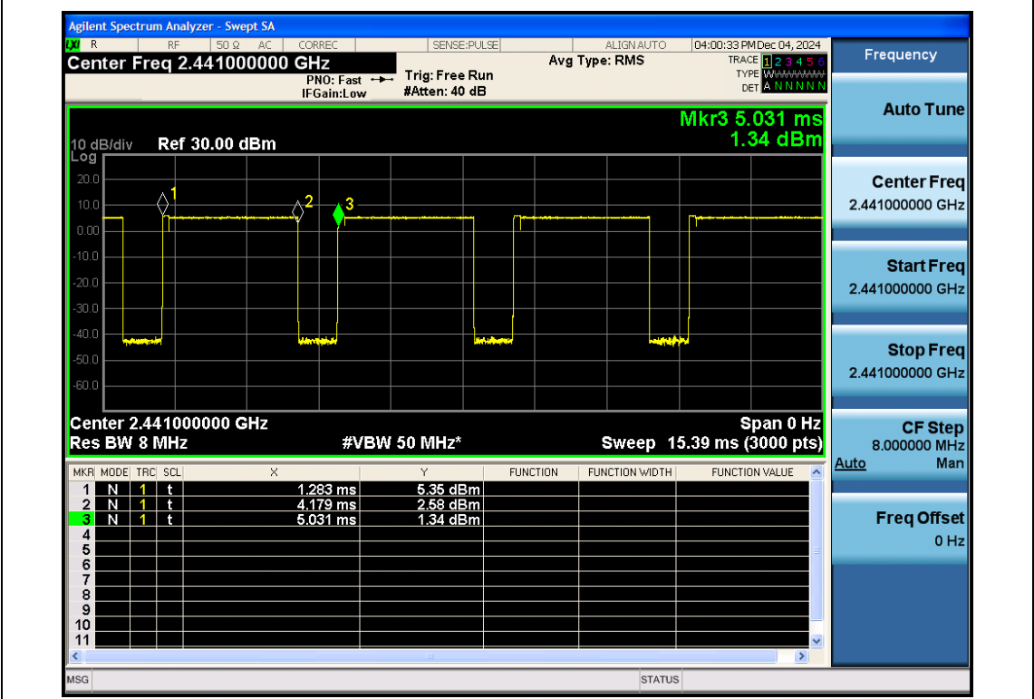
EDR-8DPSK-ANT1-2441
