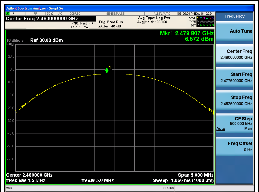
Test_Graph_BR_ANT1_2480_1Mbps_Peak Power
