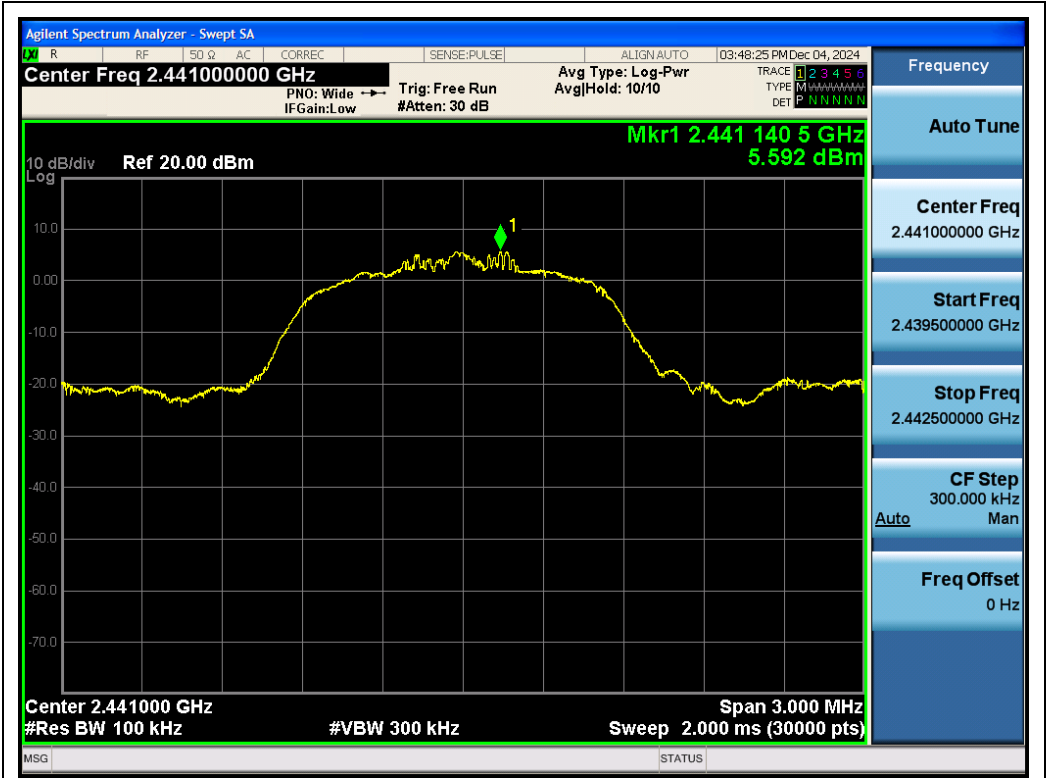
Test_Graph_EDR_ANT1_2441_2Mbps_Reference Level
