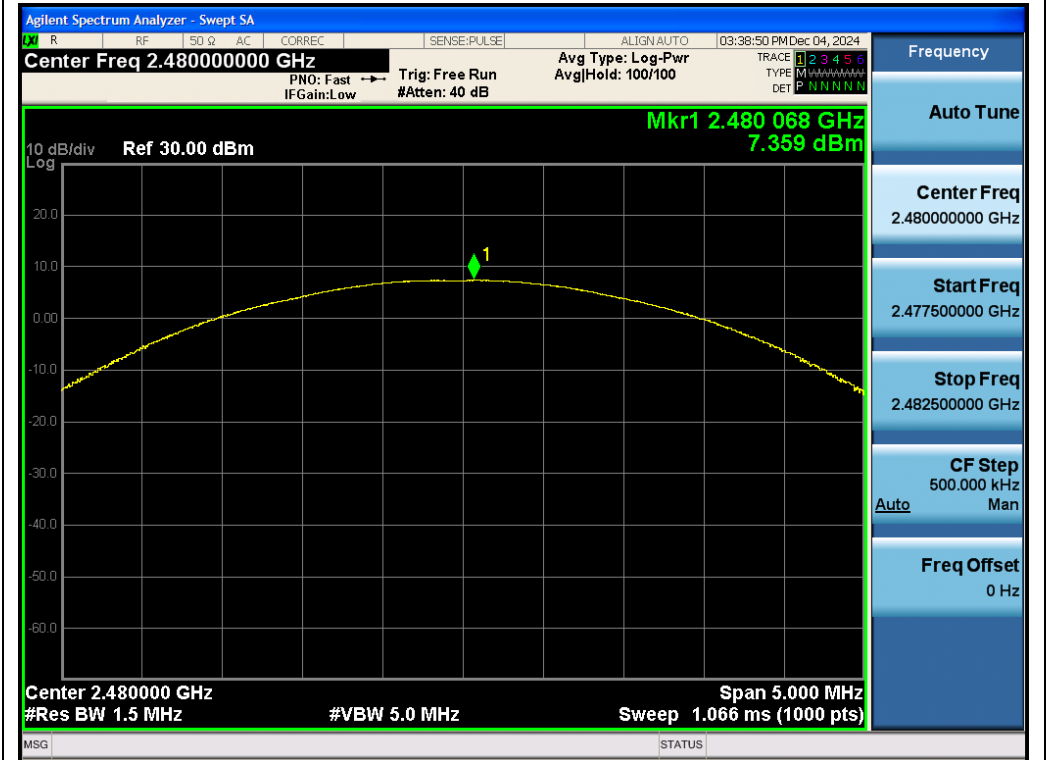
Test_Graph_EDR_ANT1_2480_2Mbps_Peak Power
