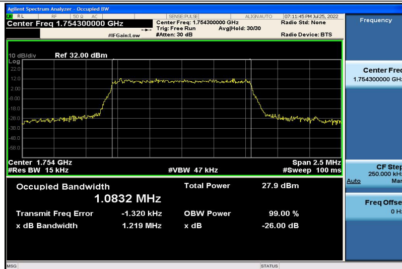
Band4-1.4MHz-16QAM-20393-6RB#0-1.0832
