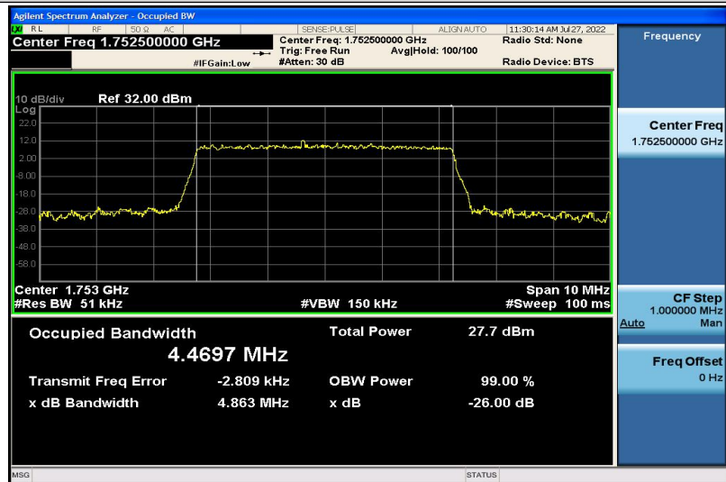
Band4-5MHz-16QAM-20375-25RB#0-4.4697
