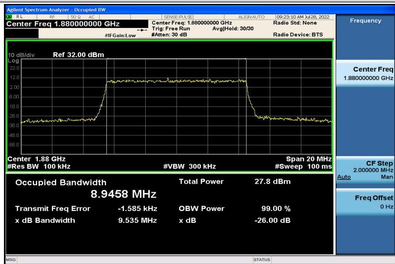
Band2-10MHz-16QAM-18900-50RB#0-8.9458
