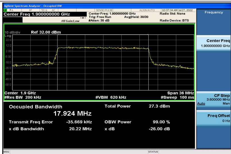
Band2-20MHz-QPSK-19100-100RB#0-17.924
