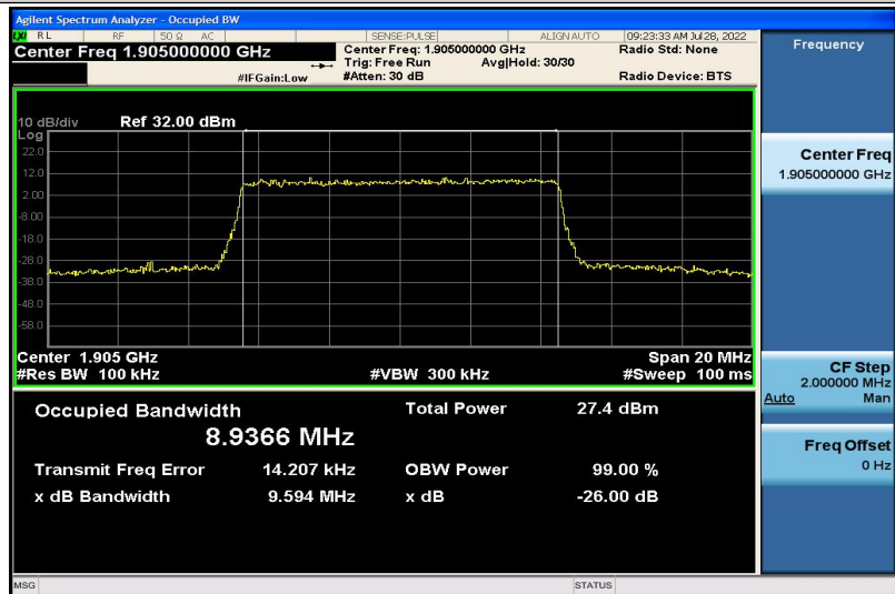
Band2-10MHz-16QAM-19150-50RB#0-8.9366
