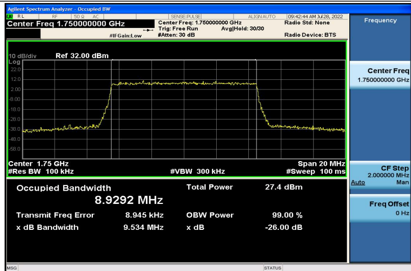
Band4-10MHz-16QAM-20350-50RB#0-8.9292
