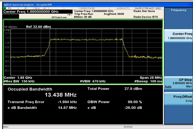
Band2-15MHz-16QAM-18900-75RB#0-13.438
