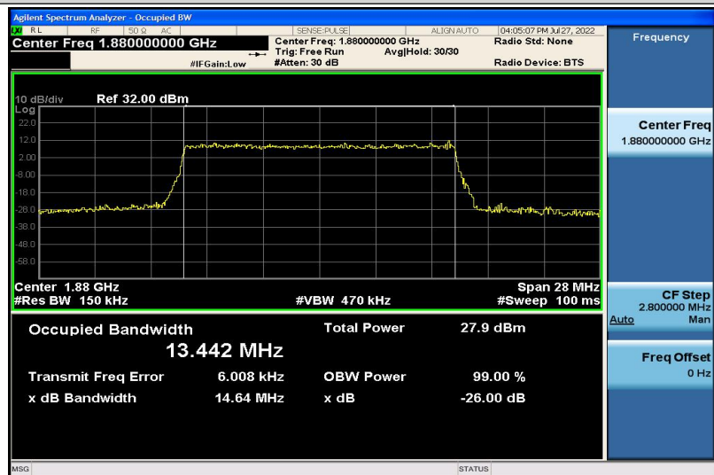
Band2-15MHz-QPSK-18900-75RB#0-13.442
