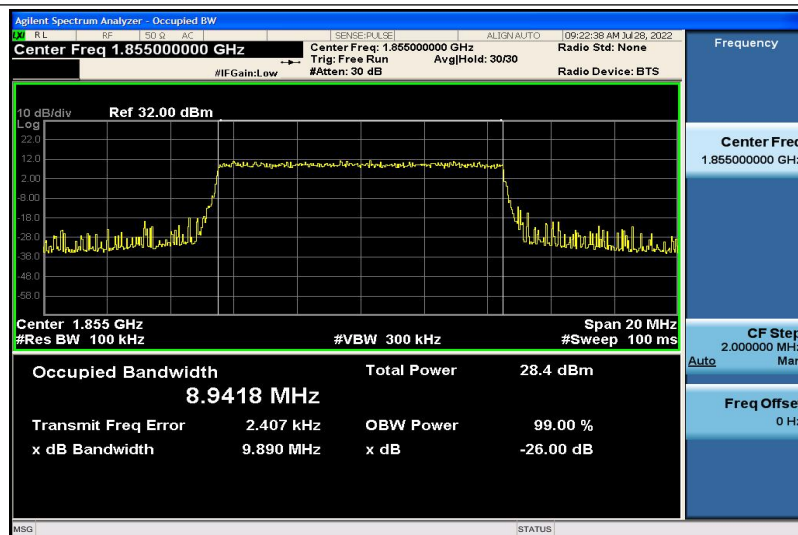
Band2-10MHz-QPSK-18650-50RB#0-8.9418
