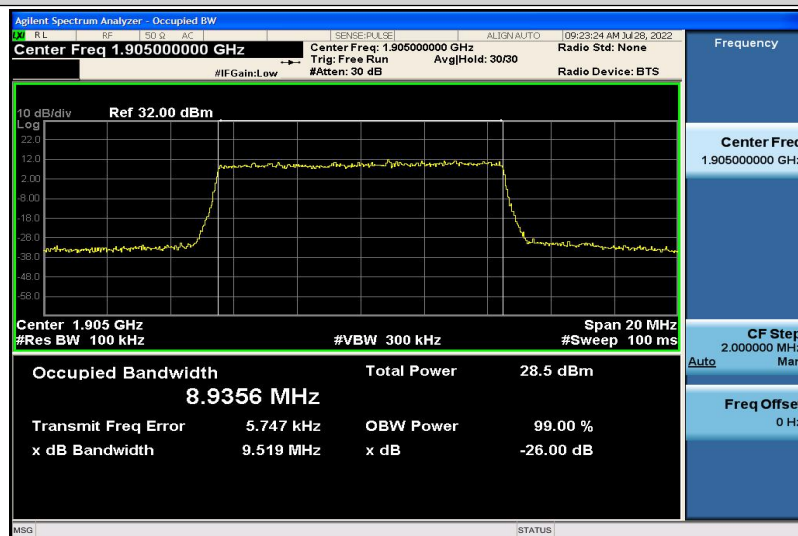
Band2-10MHz-QPSK-19150-50RB#0-8.9356
