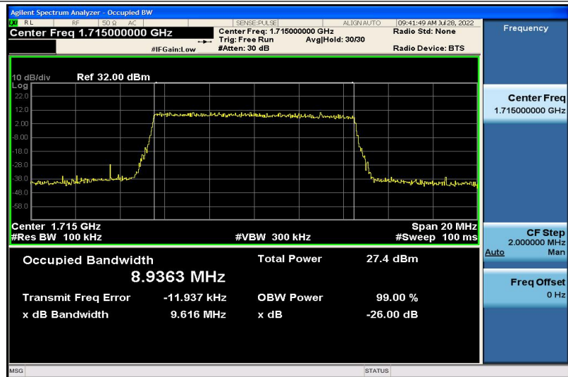
Band4-10MHz-QPSK-20000-50RB#0-8.9363
