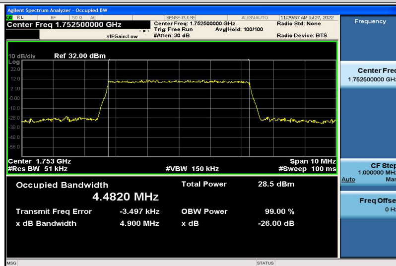
Band4-5MHz-QPSK-20375-25RB#0-4.4820
