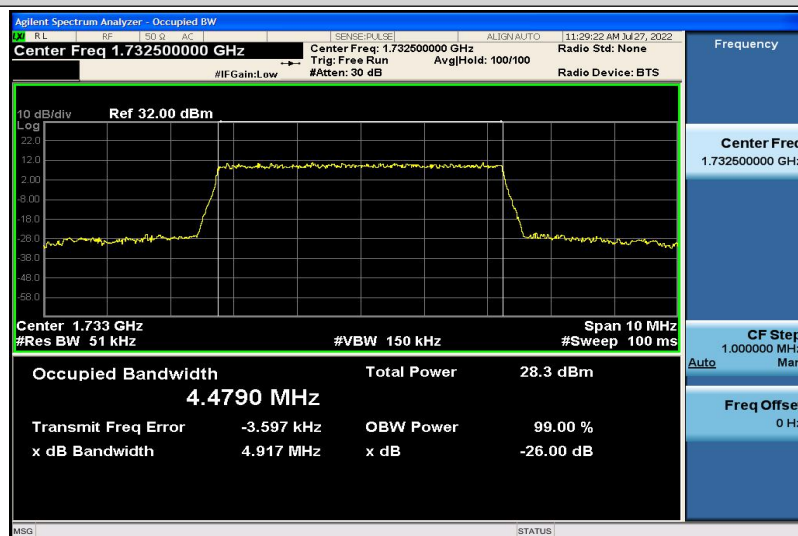
Band4-5MHz-QPSK-20175-25RB#0-4.4790
