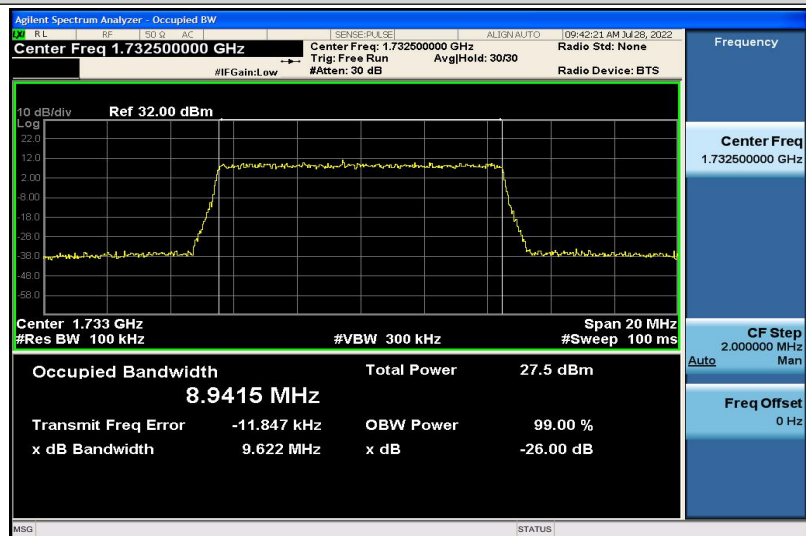
Band4-10MHz-16QAM-20175-50RB#0-8.9415
