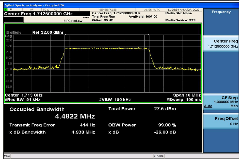
Band4-5MHz-16QAM-19975-25RB#0-4.4822
