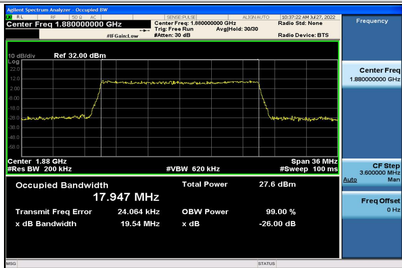
Band2-20MHz-16QAM-18900-100RB#0-17.947
