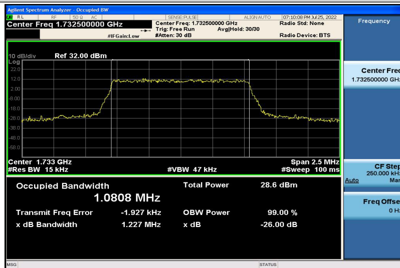
Band4-1.4MHz-QPSK-20175-6RB#0-1.0808
