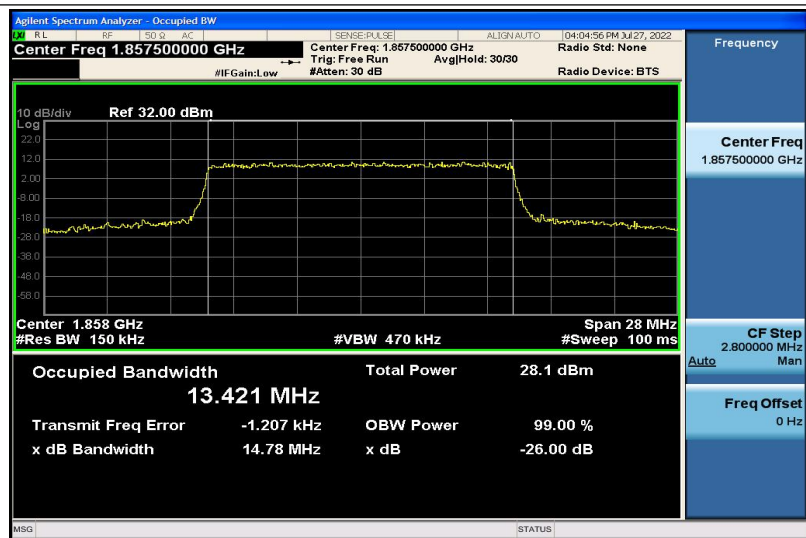
Band2-15MHz-16QAM-18675-75RB#0-13.421
