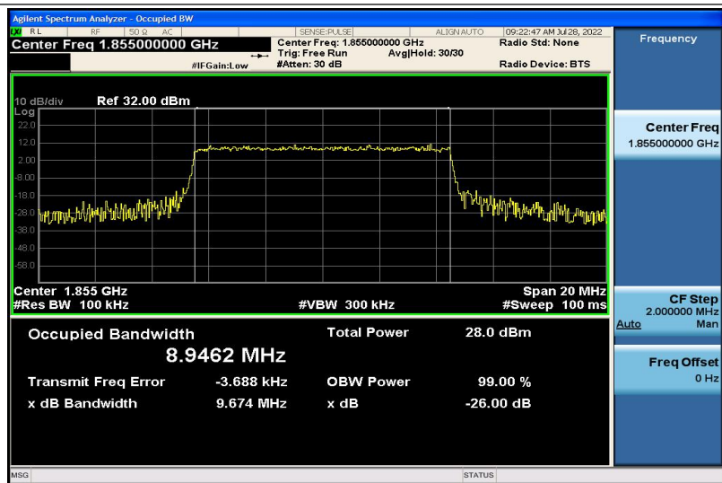
Band2-10MHz-16QAM-18650-50RB#0-8.9462
