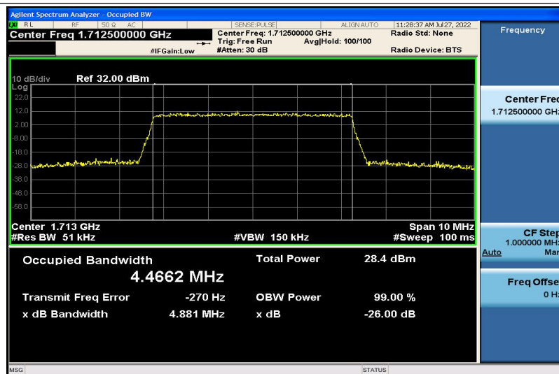
Band4-5MHz-QPSK-19975-25RB#0-4.4662
