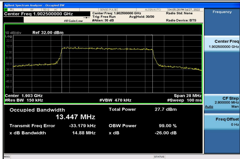
Band2-15MHz-QPSK-19125-75RB#0-13.447
