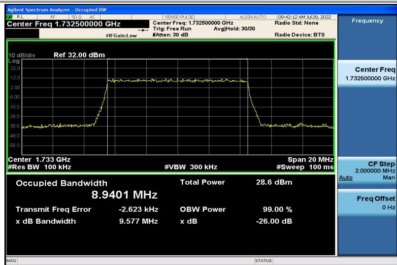
Band4-10MHz-QPSK-20175-50RB#0-8.9401
