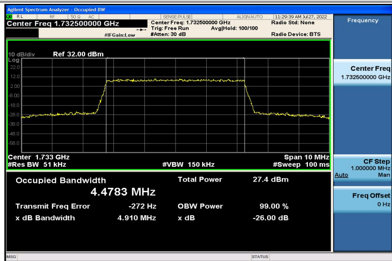
Band4-5MHz-16QAM-20175-25RB#0-4.4783
