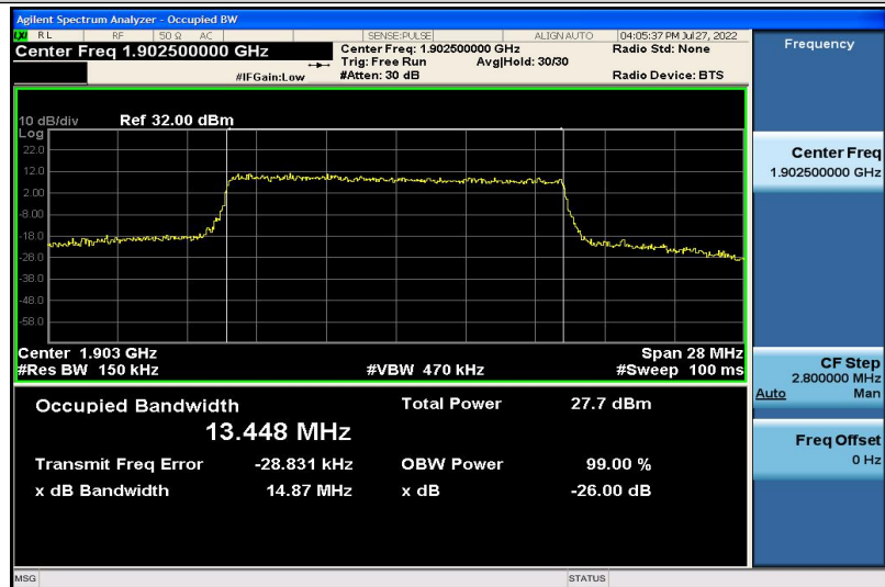
Band2-15MHz-16QAM-19125-75RB#0-13.448
