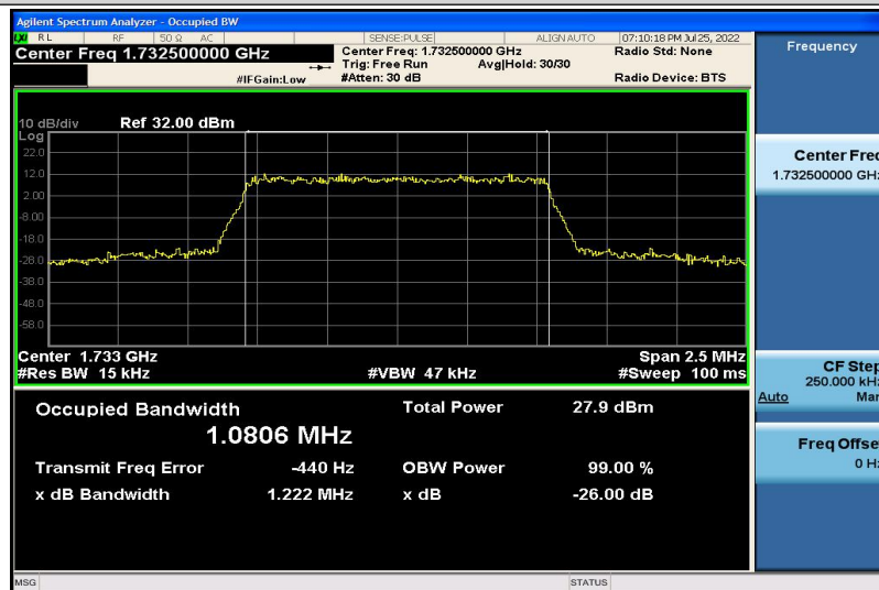
Band4-1.4MHz-16QAM-20175-6RB#0-1.0806
