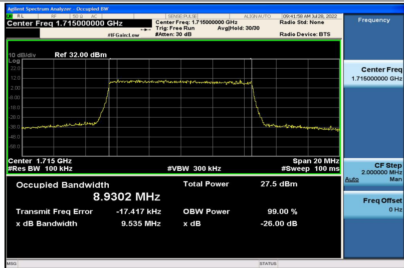
Band4-10MHz-16QAM-20000-50RB#0-8.9302
