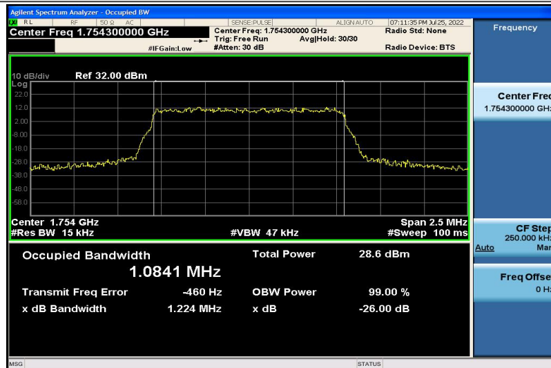
Band4-1.4MHz-QPSK-20393-6RB#0-1.0841
