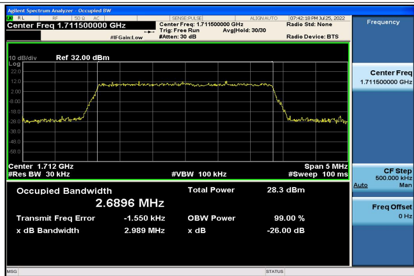
Band4-3MHz-16QAM-19965-15RB#0-2.6896
