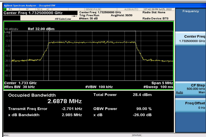
Band4-3MHz-16QAM-20175-15RB#0-2.6878
