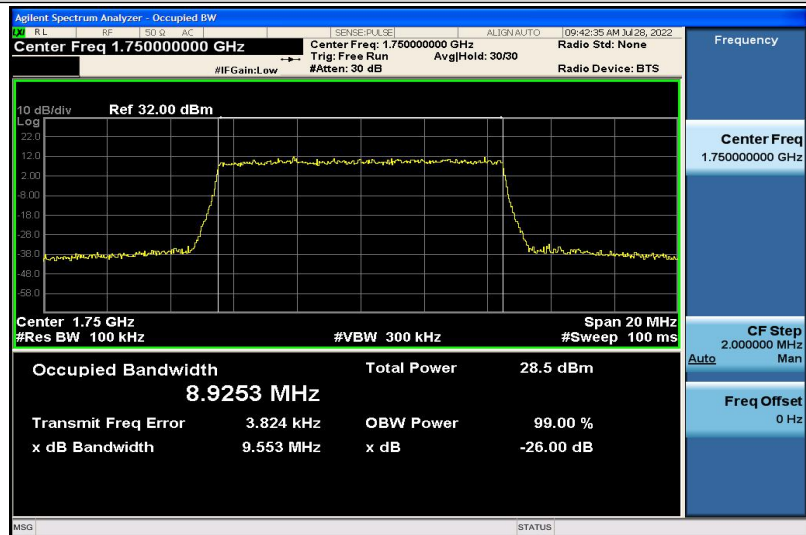
Band4-10MHz-QPSK-20350-50RB#0-8.9253
