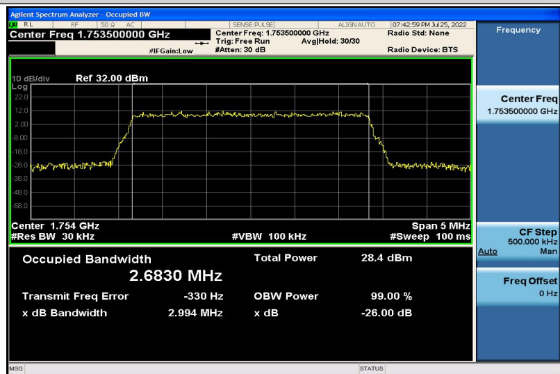
Band4-3MHz-16QAM-20385-15RB#0-2.6830
