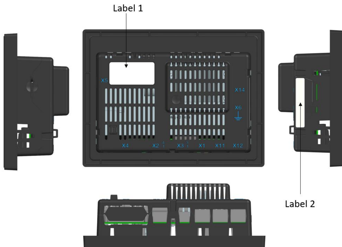
5 Figure 6-8 Connector marking SC3L
