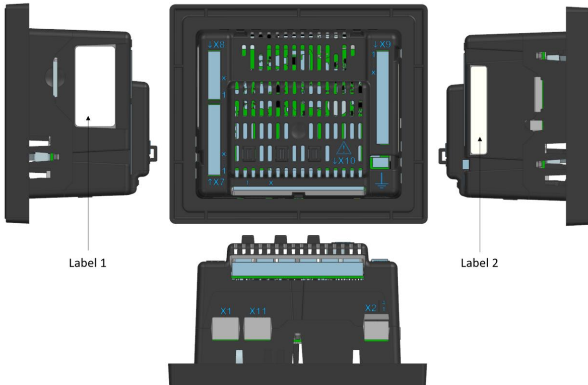
Figure 6-4 Connector marking SC3S
