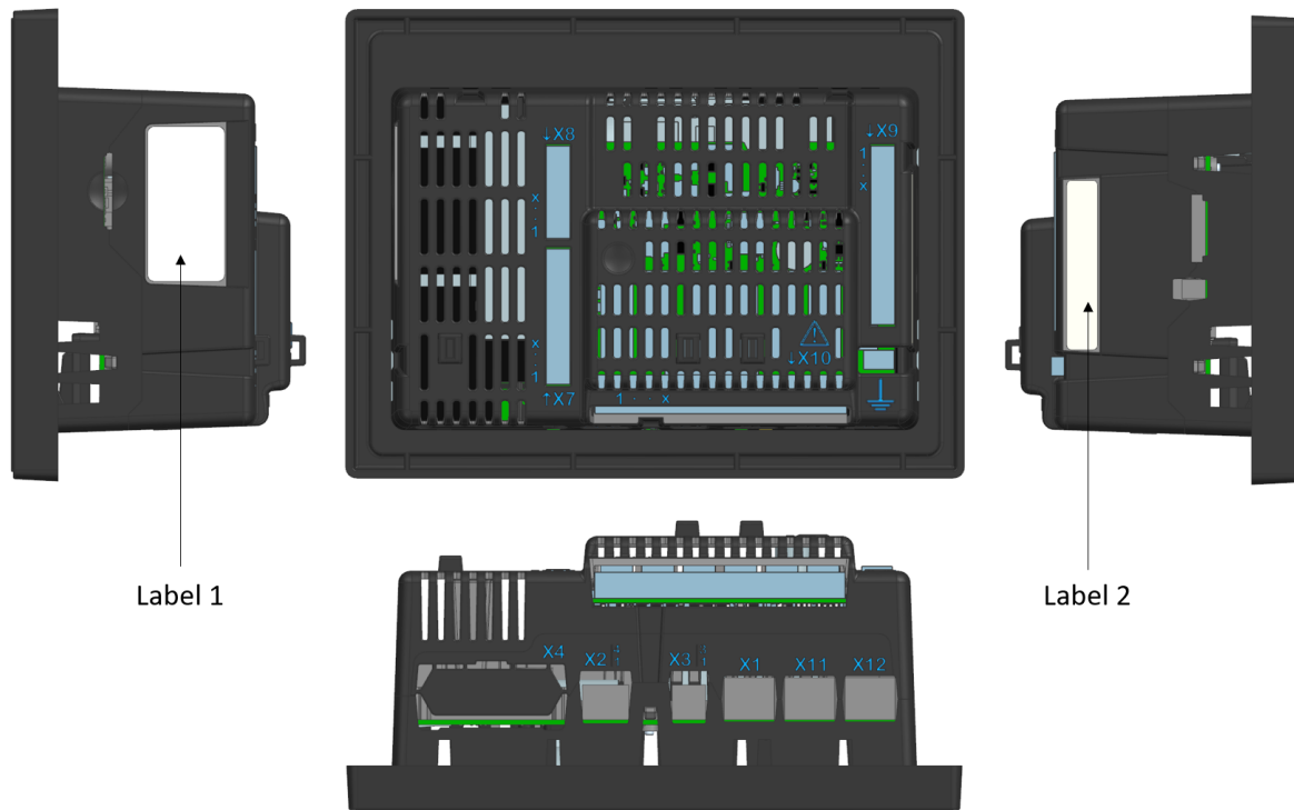
Figure 6-6 Connector marking SC3M
