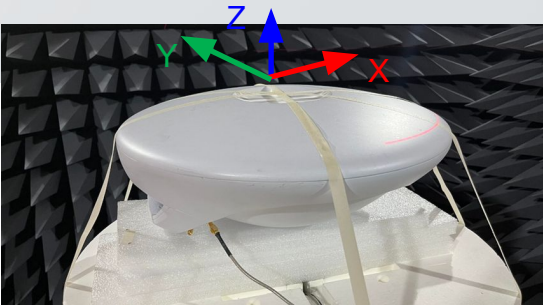
1. Antenna type: Dish 117-03751
