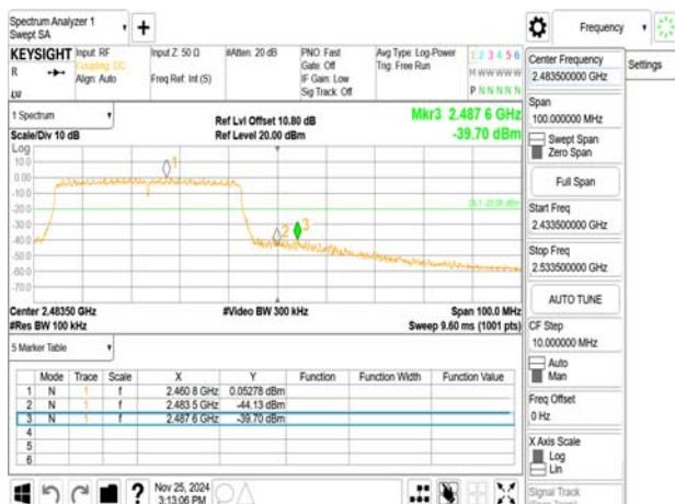
802.11ax_40MHz_Chain0_2457MHz_RU242_62
