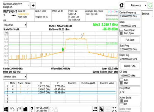
802.11ax_20MHz_Chain0_2412MHz_R242
