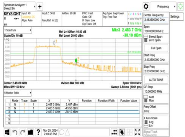
802.11ax_20MHz_Chain0_2462MHz_R242
