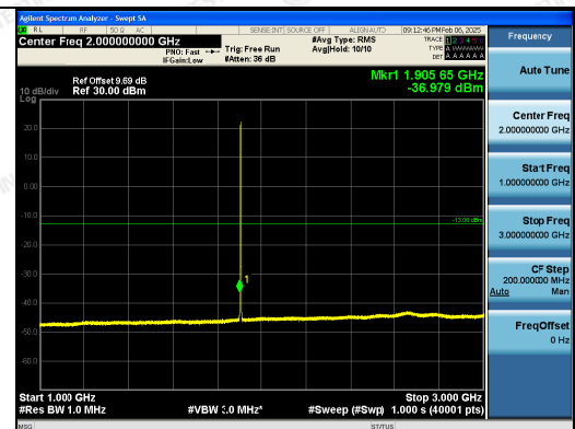
1GHz~3GHz
