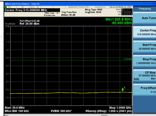
30MHz~1GHz
