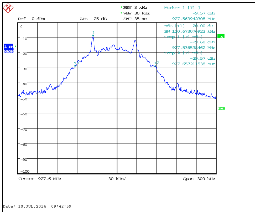
Fc = 927.6 MHz - 20dB Bandwidth
