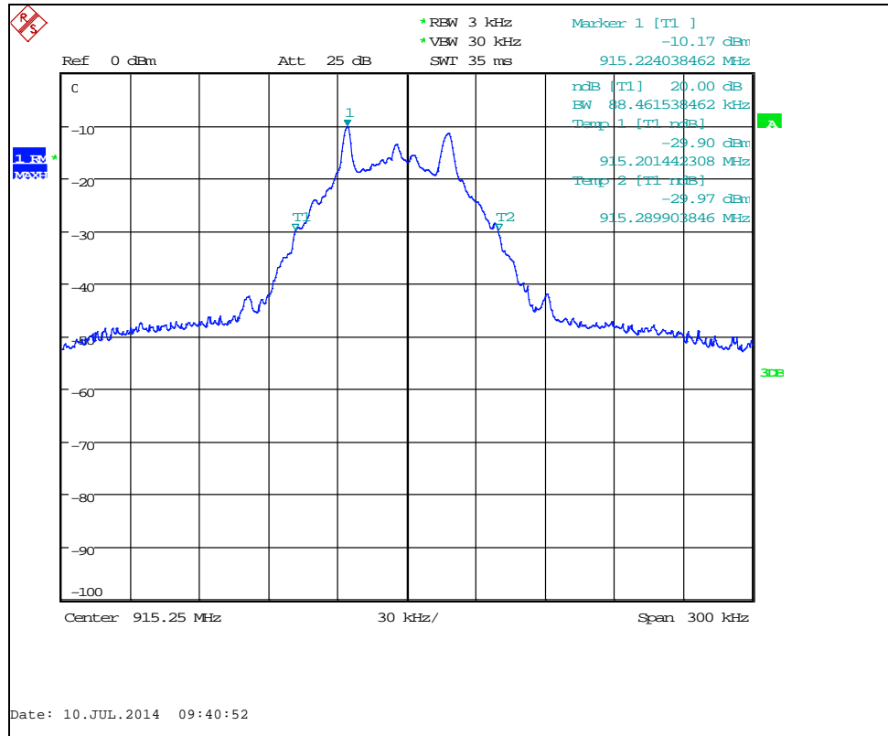
Fc = 915.25 MHz - 20dB Bandwidth
