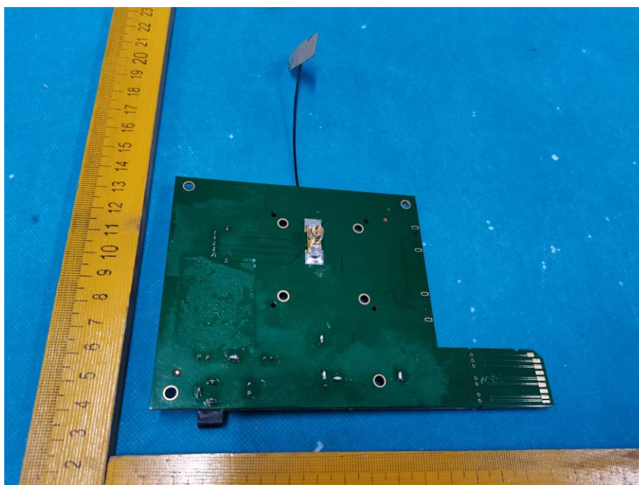
Fig.2 Eut in Test Fixture
