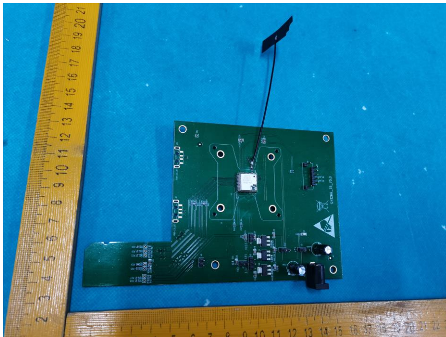
Fig.1 Eut in Test Fixture
