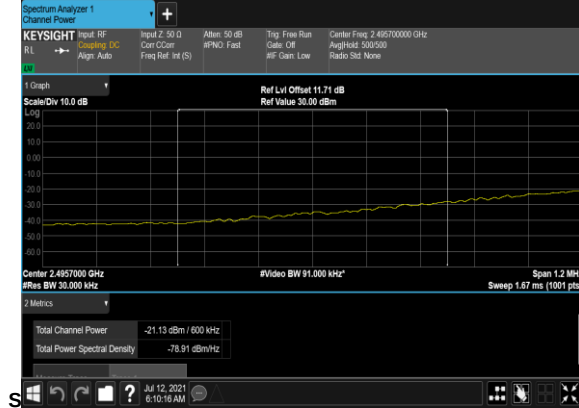
N41(60M)_DFT-s- OFDM_QPSK_Edge_1RB_Left_Low_CH_chp_PAS
