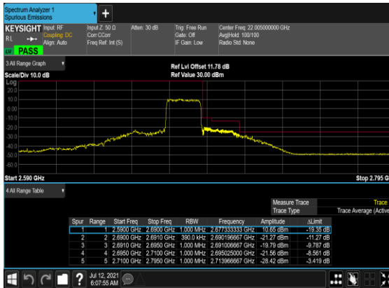
N41(20M)_DFT-s- OFDM_QPSK_Outer_Full_High_CH
