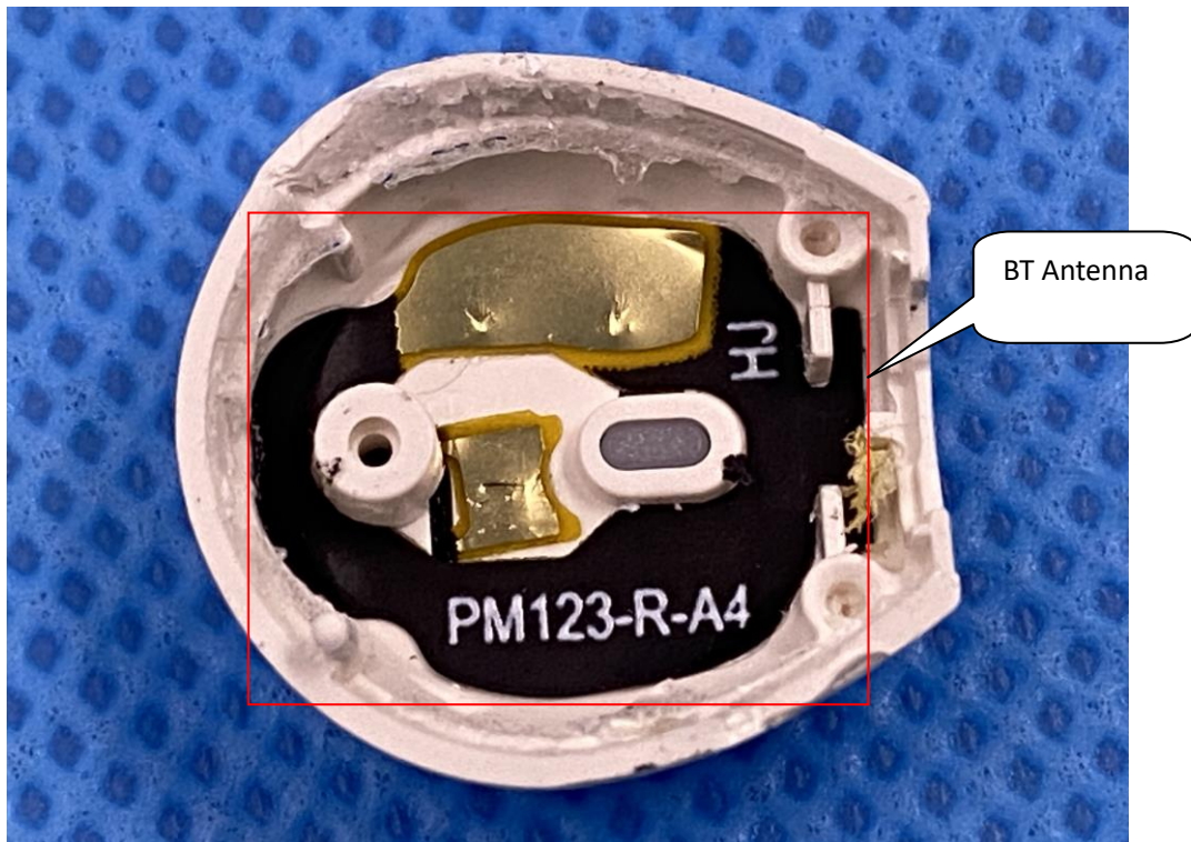
OPEN VIEW OF EUT (FIGURE 2)
