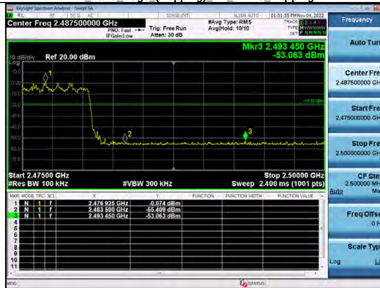
2 Band Edge (Hopping) BT 2-DH5 Hopping
