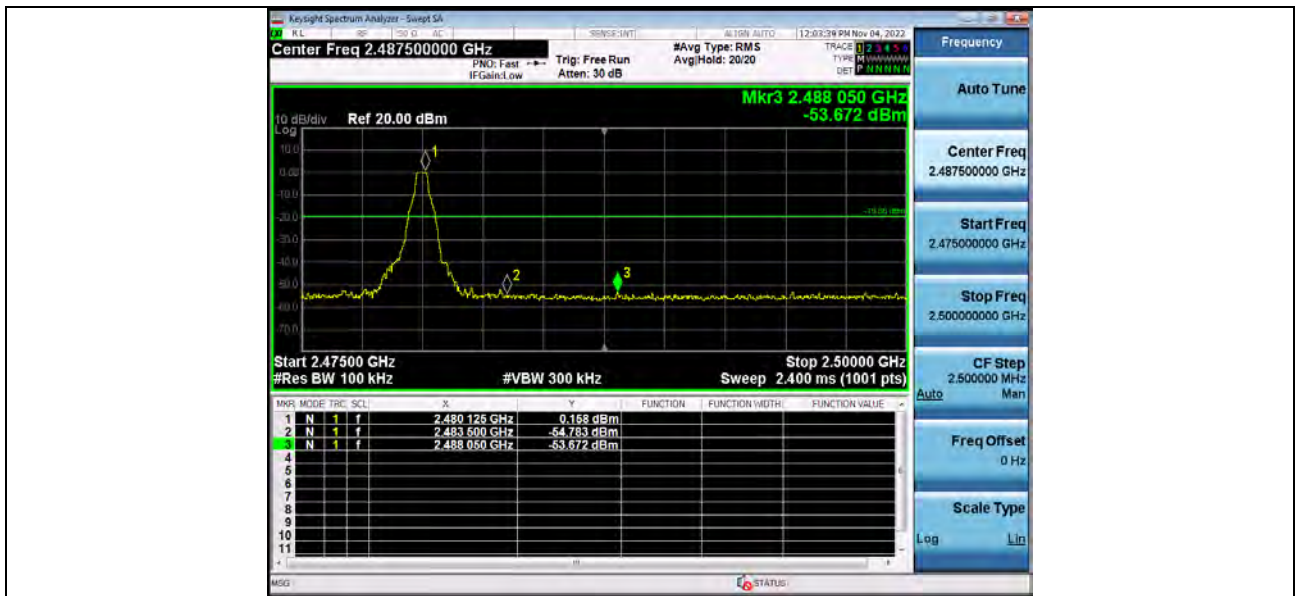
1 Reference Level BT 1-DH5 Hopping
