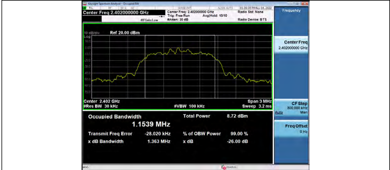
99% Occupied Bandwidth BT 2-DH5 2402
