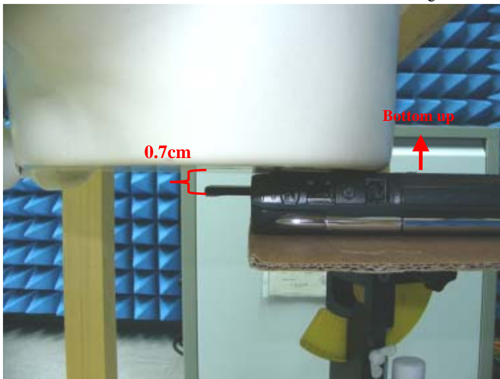
Fig.8 Photograph of the top cover parallel and at a distance of 0.0 cm from the base of the phantom. (0.7 cm Spacing between EUT & Planar Phantom)
