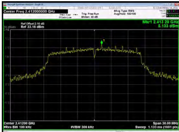
802.11g, Channel No.: 1
