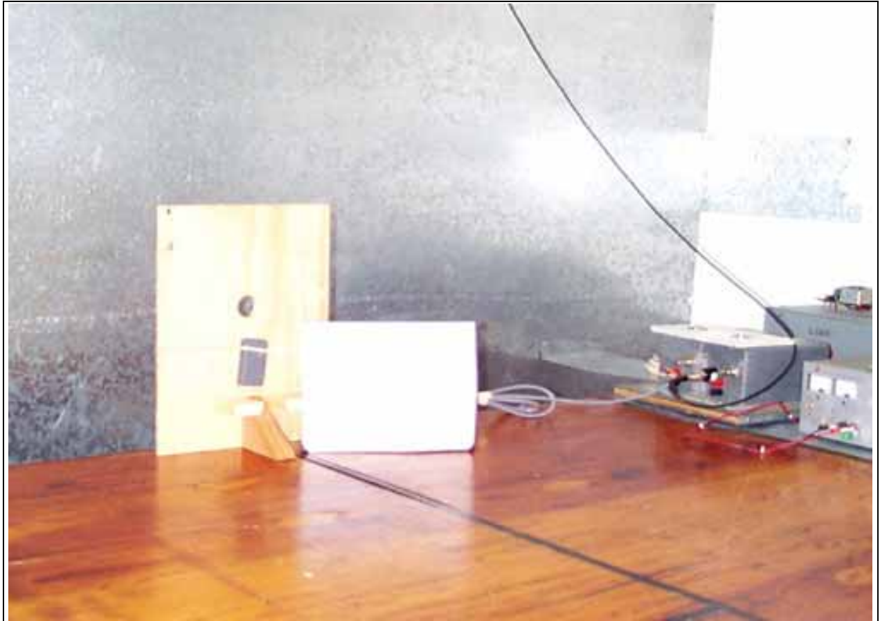
AC Conducted Emissions - Front View of the 6005/8B (6005-310)
