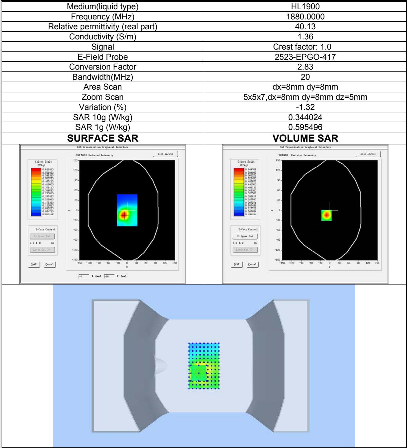
Plot 5: LTE BAND 2, Middle channel (Body-worn, Front Side) Product Description:LTE MiFi Router Test Date: 2024-03-28
