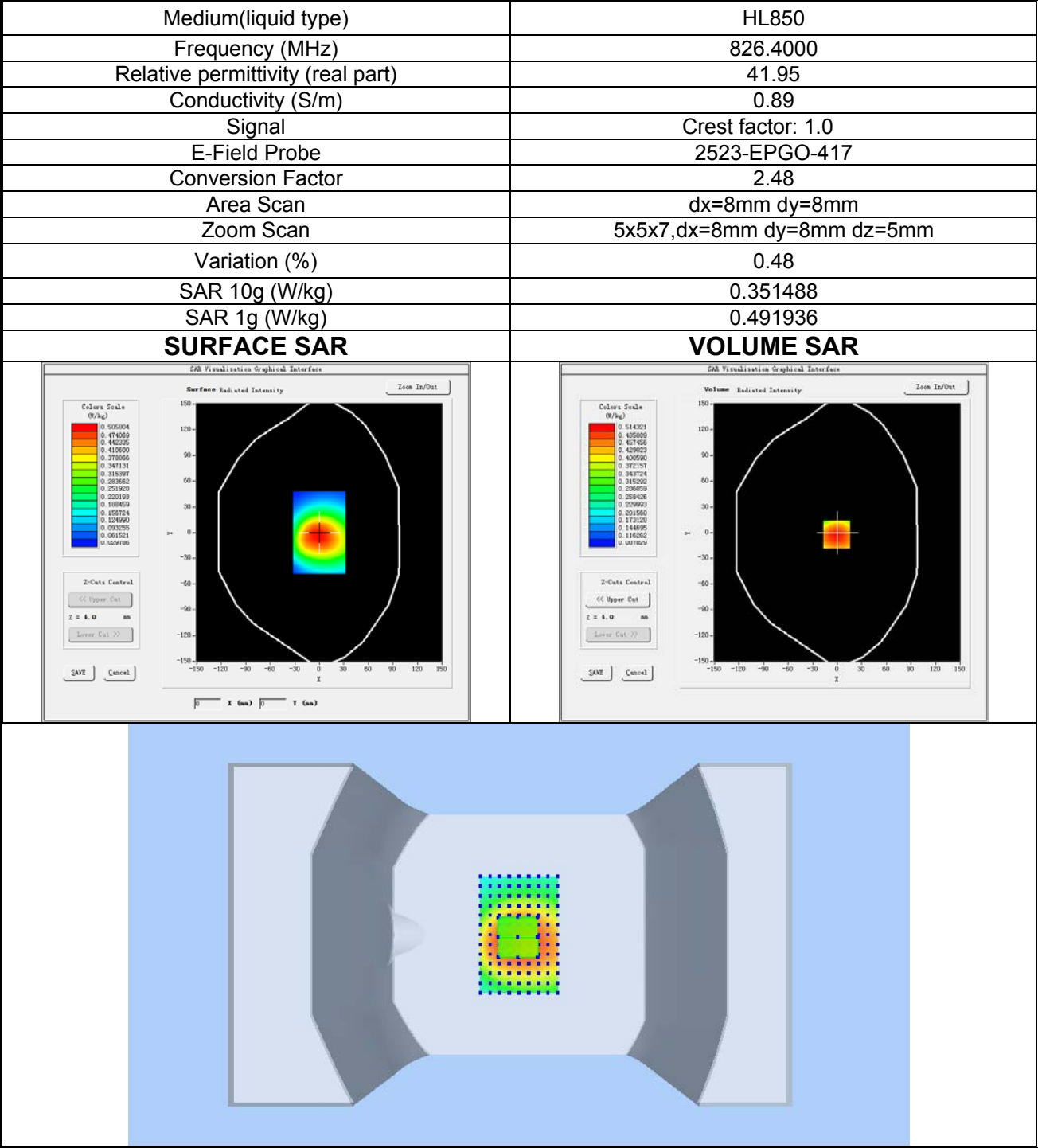
Plot 4: WCDMA BAND V, Low channel (Body-worn, Front Side) Product Description: LTE MiFi Router Test Date: 2024-03-27
