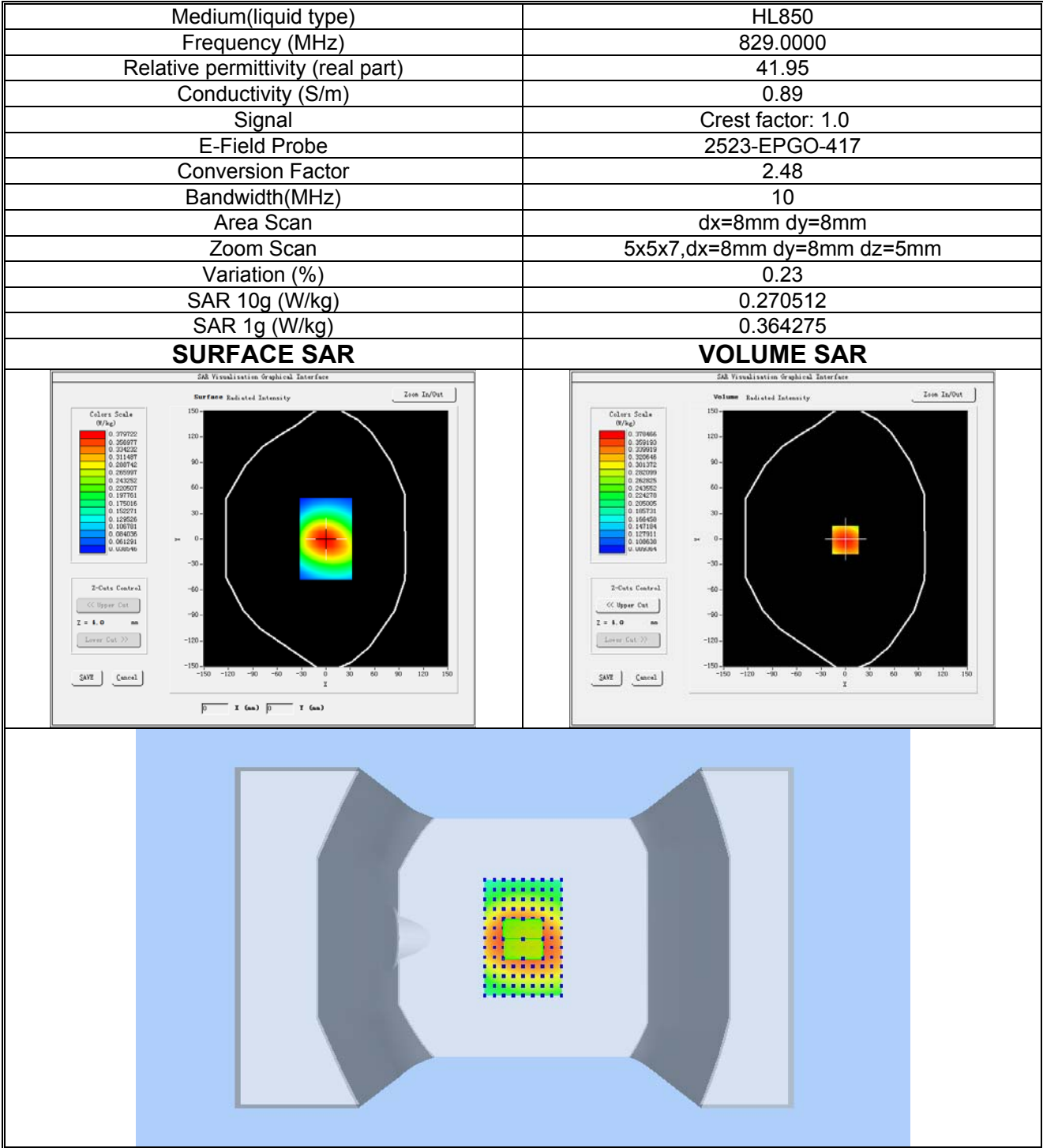
Plot 7: LTE BAND 5, Low channel (Body-worn, Front Side) Product Description: LTE MiFi Router Test Date: 2024-03-27
