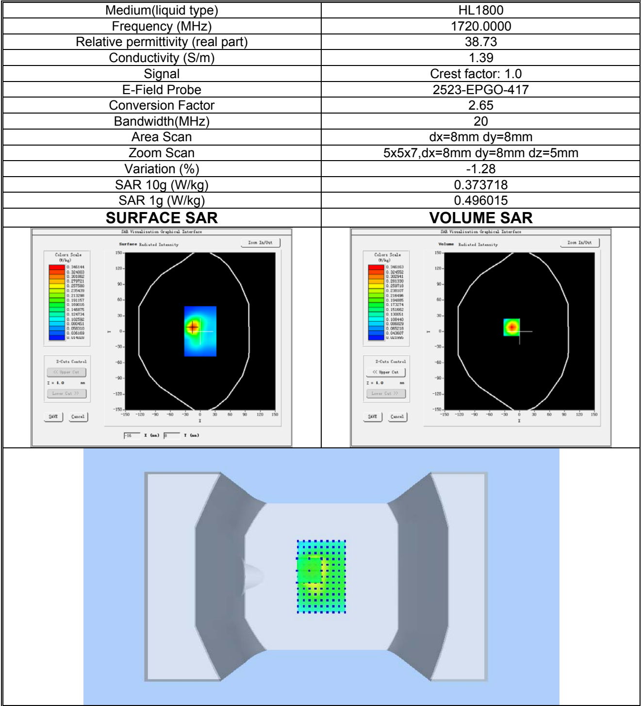
Plot 10: LTE BAND 66, Low channel (Body-worn, Front Side) Product Description: LTE MiFi Router Test Date: 2024-03-26
