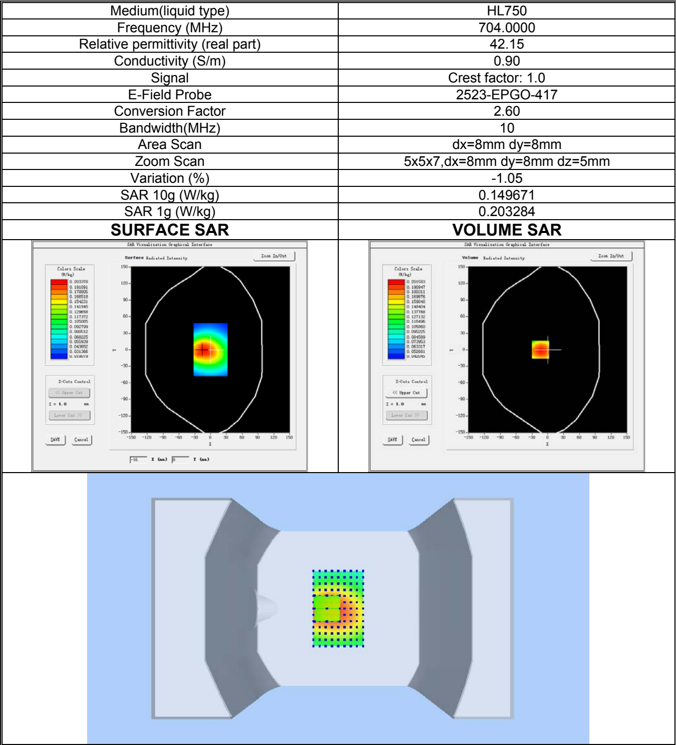
Plot 8: LTE BAND 12, Low channel (Body-worn, Front Side) Product Description: LTE MiFi Router Test Date: 2024-03-25
