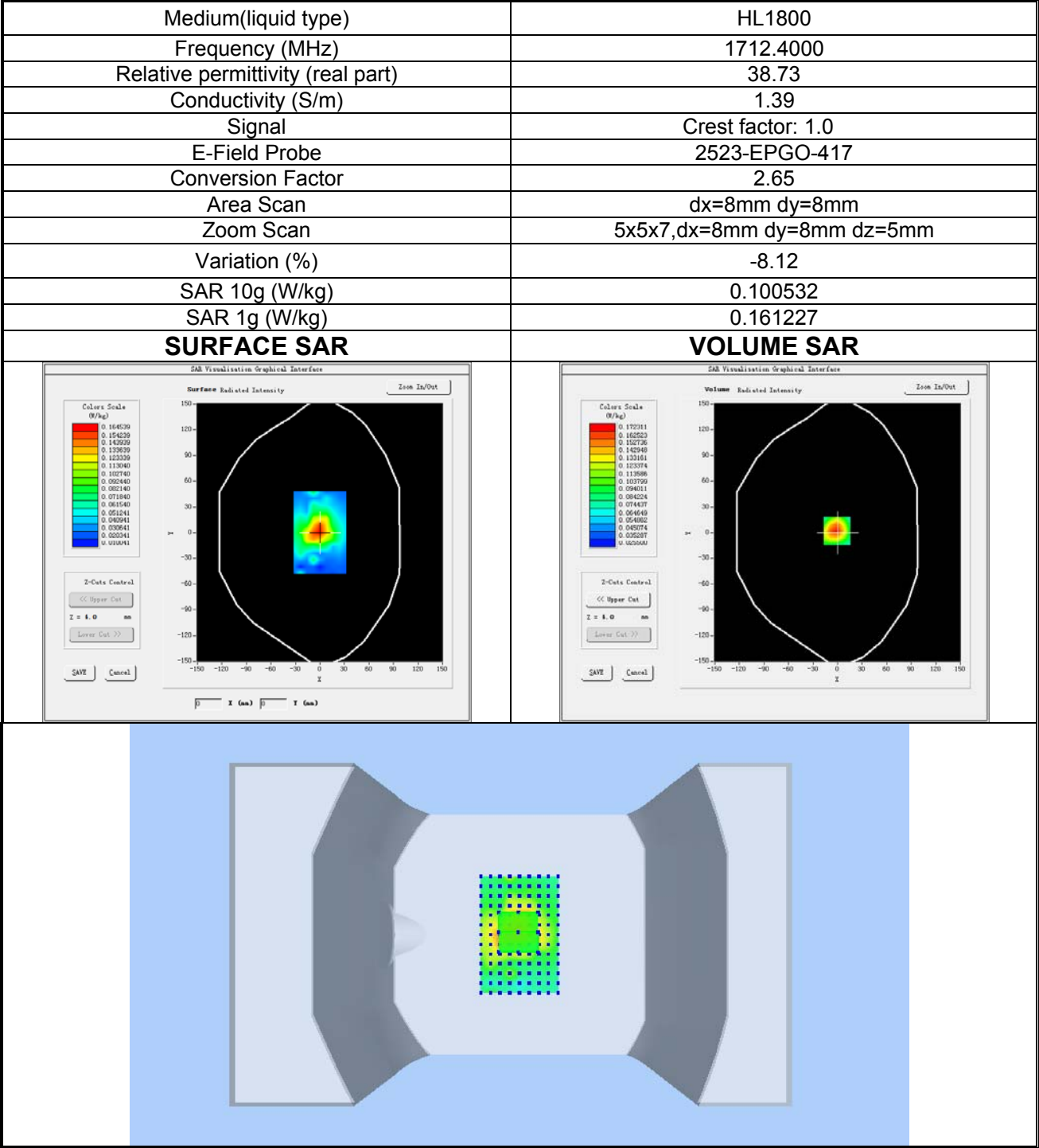
Plot 3: WCDMA BAND IV, Low channel (Body-worn, Top Edge) Product Description: LTE MiFi Router Test Date: 2024-03-26
