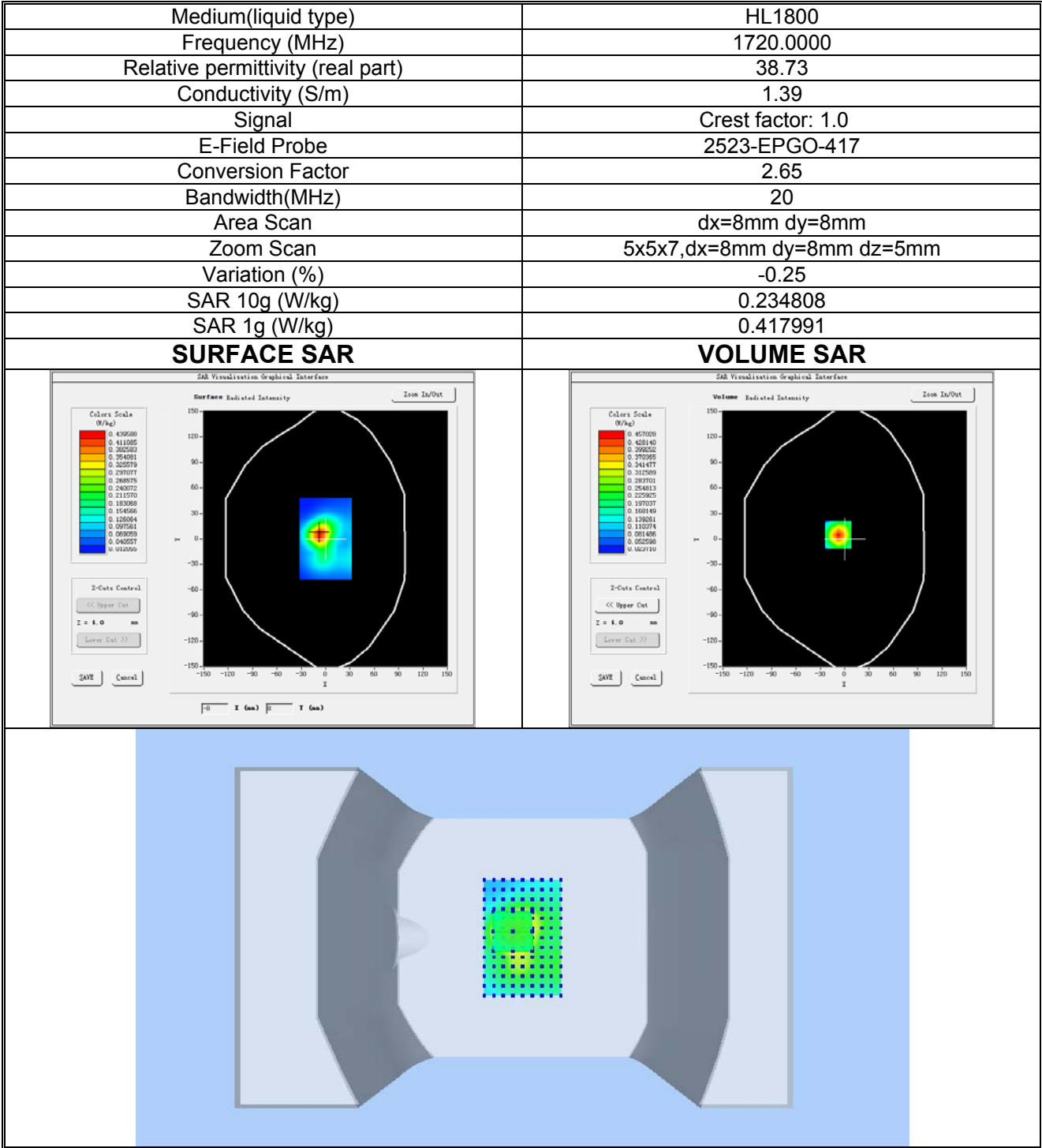
Plot 6: LTE BAND 4, Low channel (Body-worn, Front Side) Product Description: LTE MiFi Router Test Date: 2024-03-26
