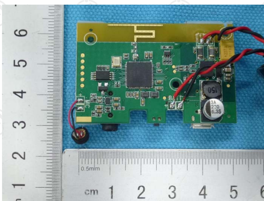
Fig.4- PCB View
