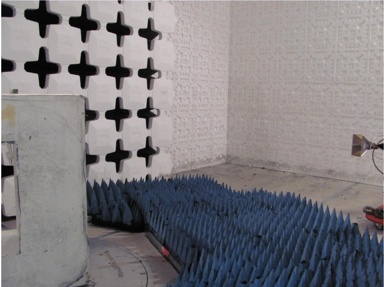
Figure 5. Radiated Emission Test Setup, EUT at 1.5 m test height
