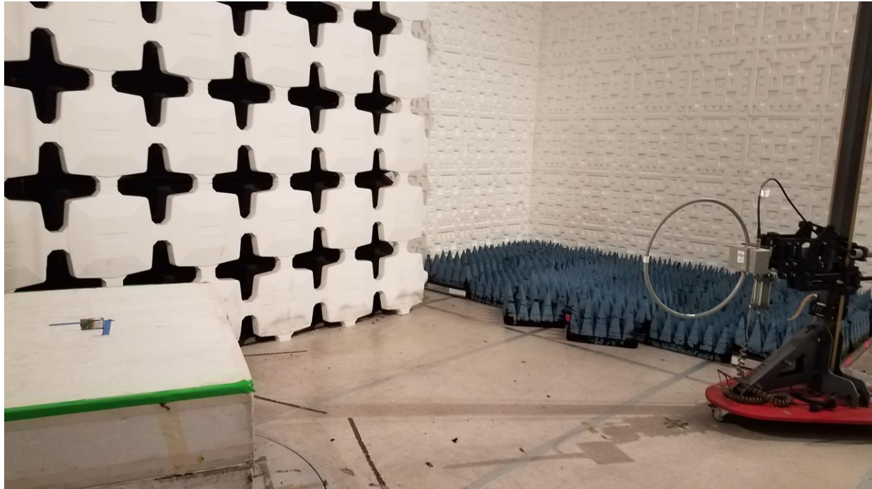
Figure 2. Radiated Emissions Test Setup, .15 MHz to 30 MHz
