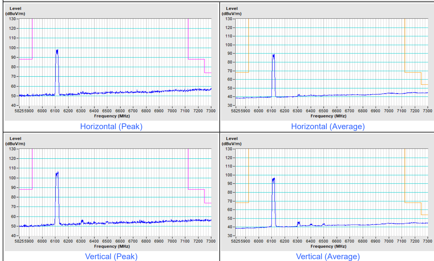
802.11a Channel 33
