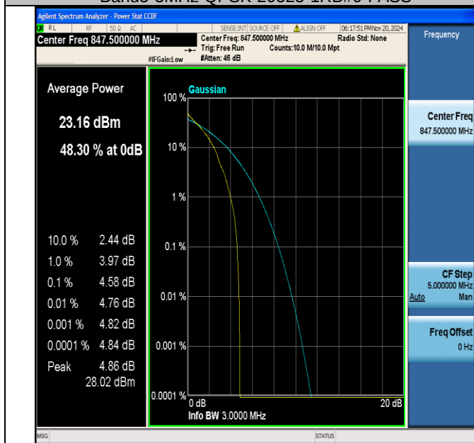
Band5-3MHz-QPSK-20635-1RB#0-PASS
