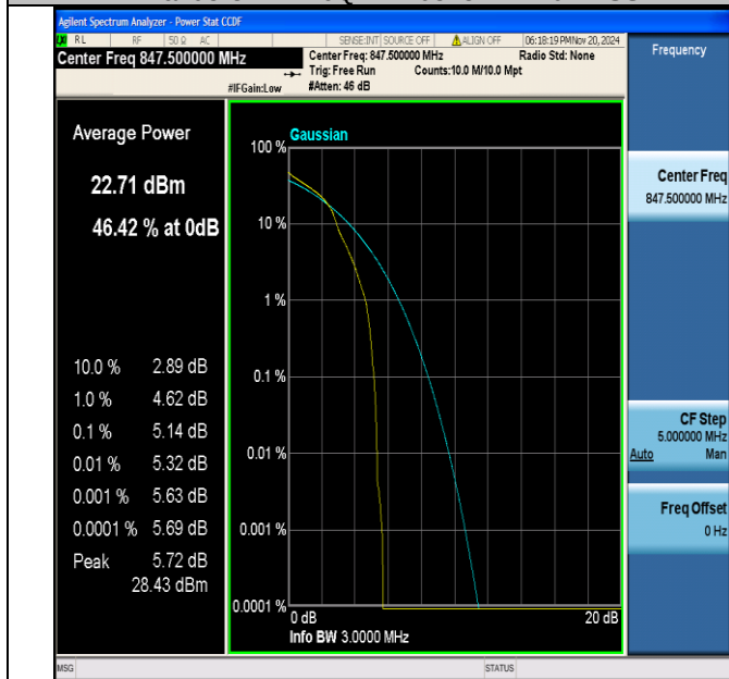
Band5-3MHz-16QAM-20635-1RB#0-PASS
