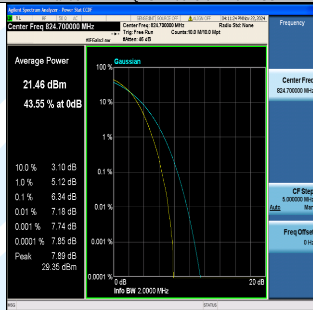
Band5-1.4MHz-64QAM-20407-6RB#0-PASS
