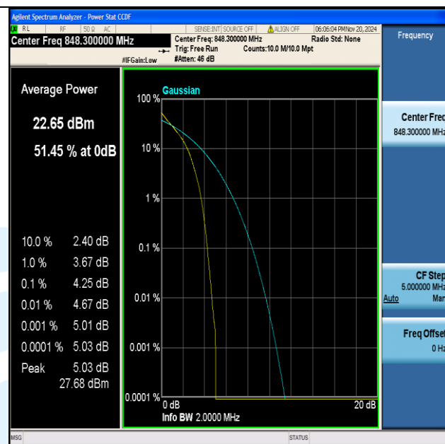
Band5-1.4MHz-QPSK-20643-6RB#0-PASS
