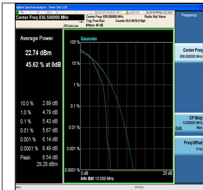
Band5-10MHz-16QAM-20525-1RB#0-PASS
