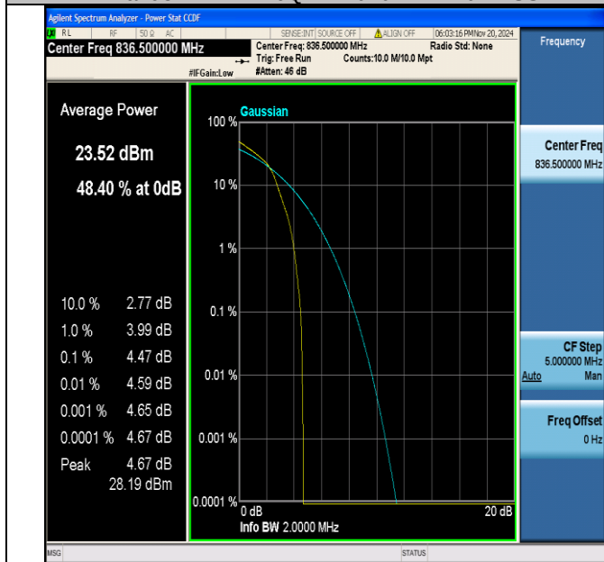
Band5-1.4MHz-16QAM-20525-1RB#0-PASS
