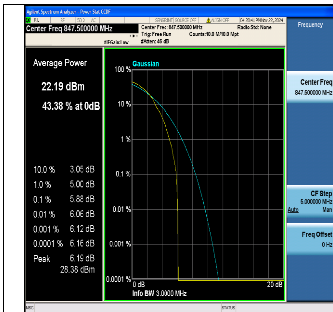
Band5-3MHz-64QAM-20635-1RB#0-PASS
