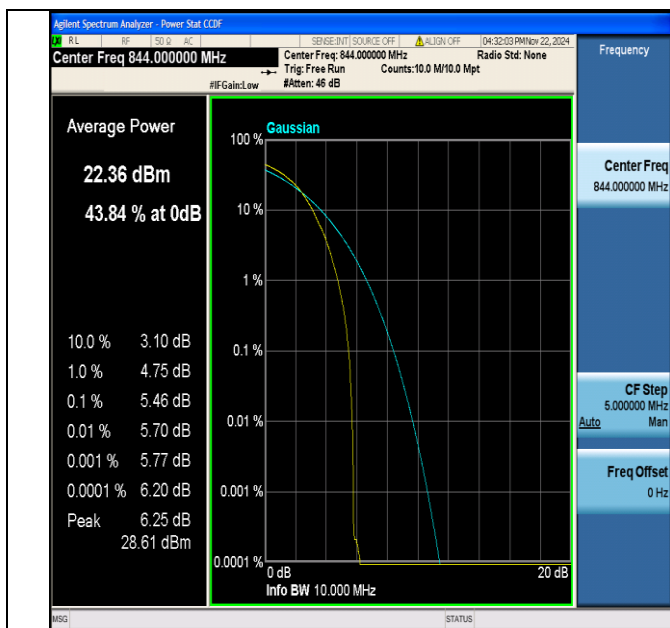
Band5-10MHz-64QAM-20600-1RB#0-PASS
