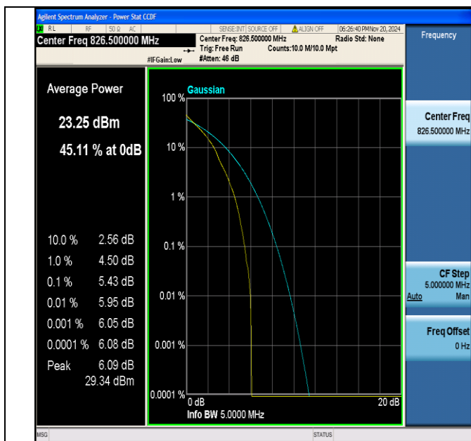
Band5-5MHz-QPSK-20425-1RB#0-PASS
