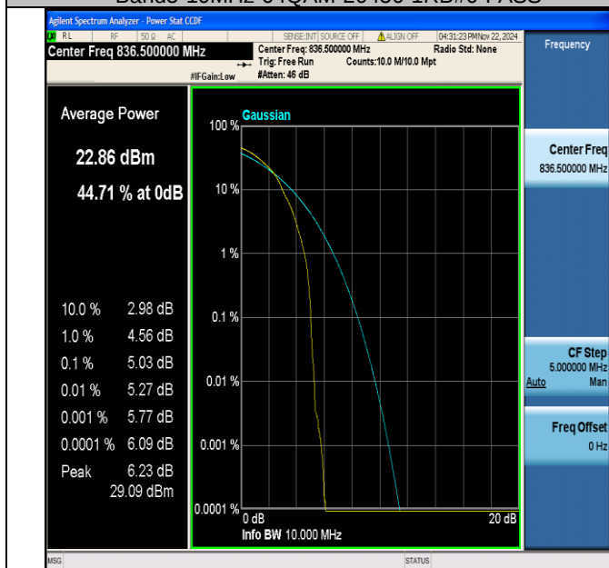
Band5-10MHz-64QAM-20525-1RB#0-PASS
