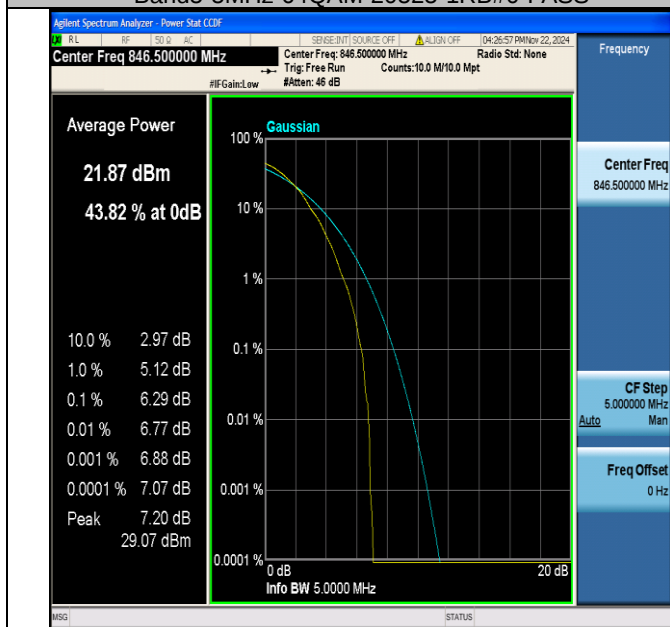
Band5-5MHz-64QAM-20625-1RB#0-PASS
