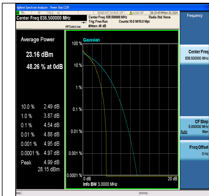
Band5-3MHz-QPSK-20525-1RB#0-PASS
