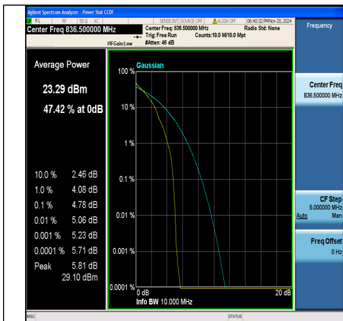
Band5-10MHz-QPSK-20525-1RB#0-PASS
