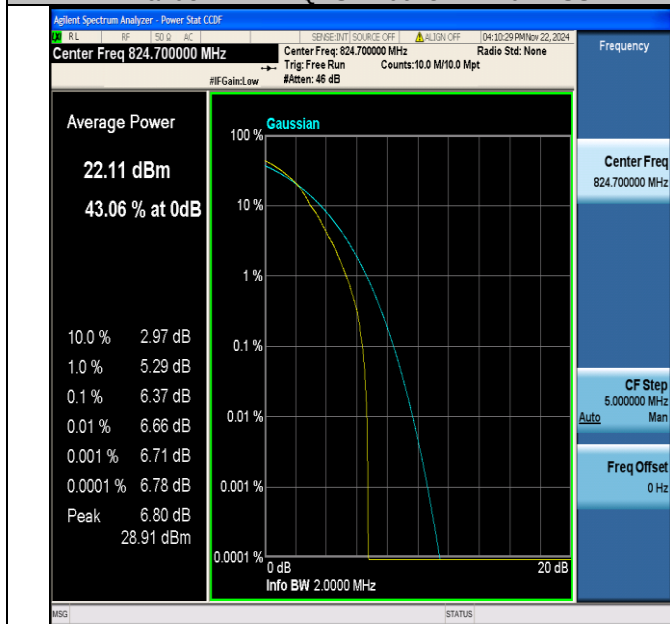
Band5-1.4MHz-64QAM-20407-1RB#0-PASS
