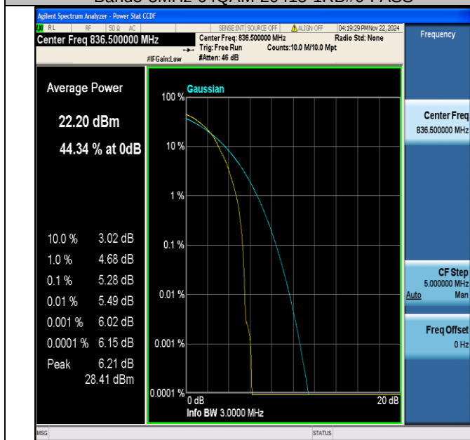
Band5-3MHz-64QAM-20525-1RB#0-PASS
