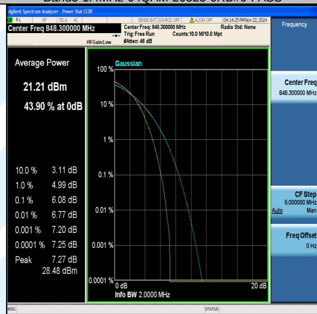
Band5-1.4MHz-64QAM-20643-6RB#0-PASS
