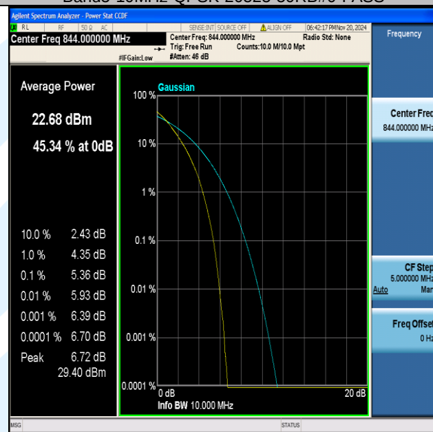
Band5-10MHz-QPSK-20600-50RB#0-PASS
