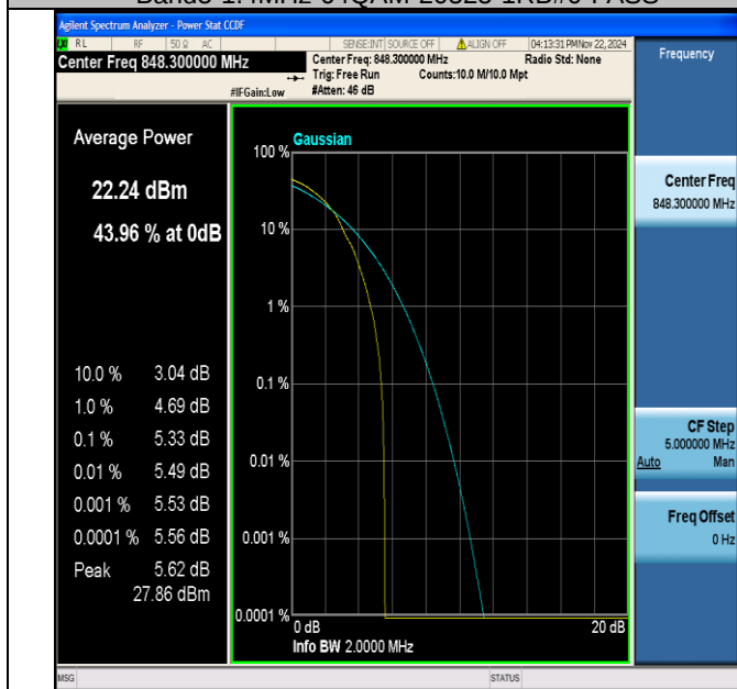
Band5-1.4MHz-64QAM-20643-1RB#0-PASS
