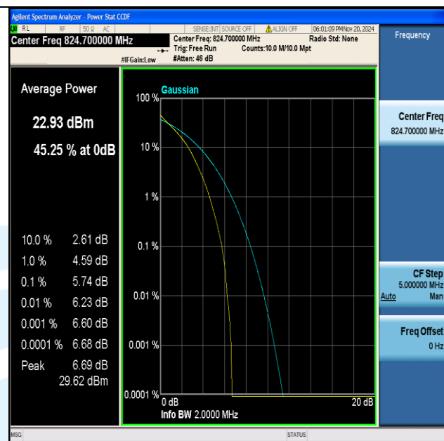
Band5-1.4MHz-QPSK-20407-6RB#0-PASS
