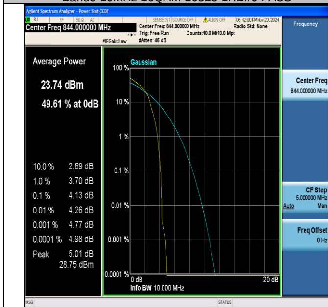
Band5-10MHz-16QAM-20600-1RB#0-PASS
