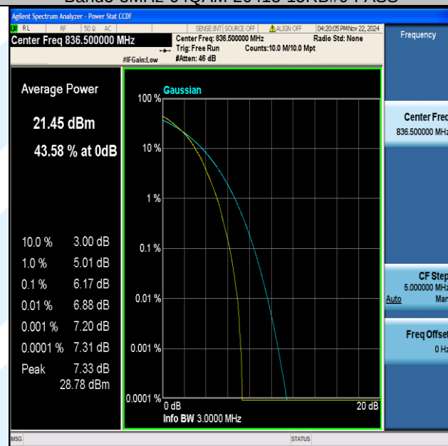
Band5-3MHz-64QAM-20525-15RB#0-PASS
