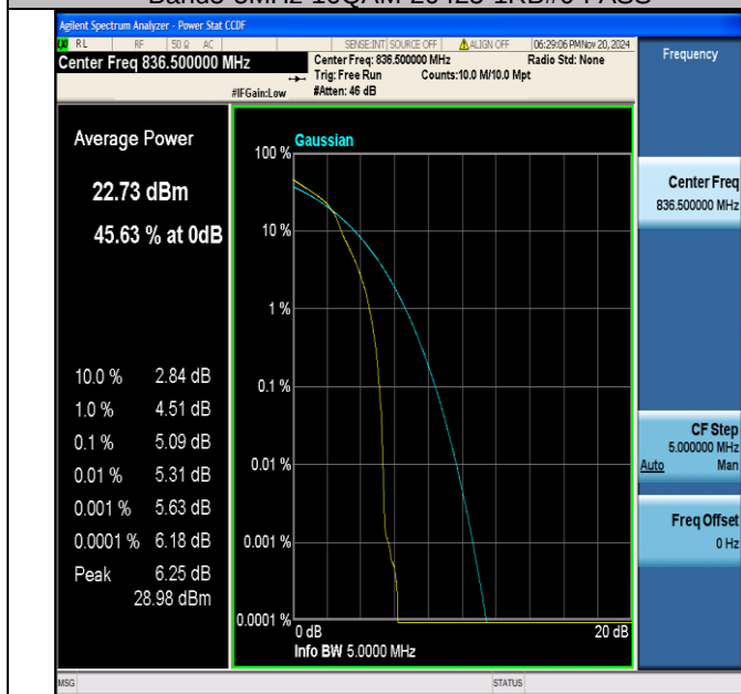
Band5-5MHz-16QAM-20525-1RB#0-PASS
