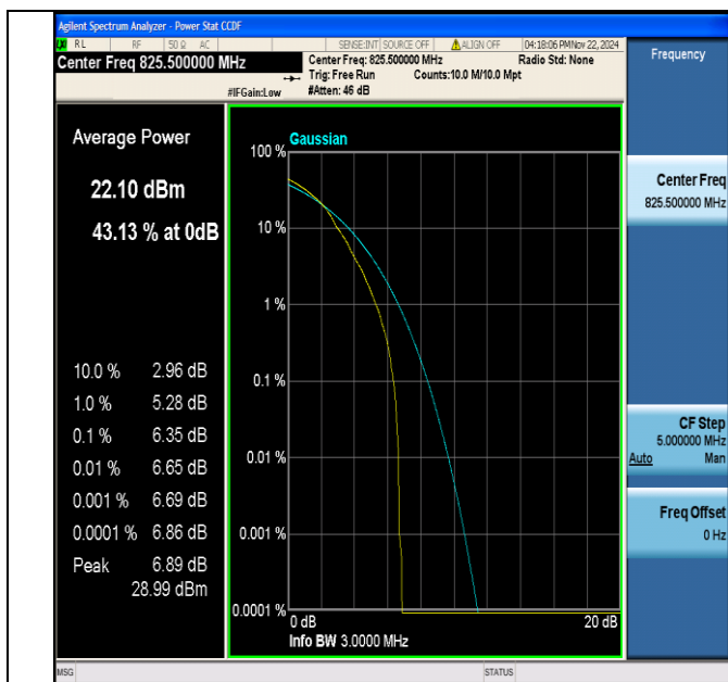
Band5-3MHz-64QAM-20415-1RB#0-PASS
