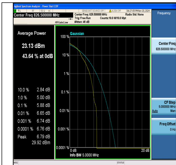
Band5-5MHz-16QAM-20425-1RB#0-PASS
