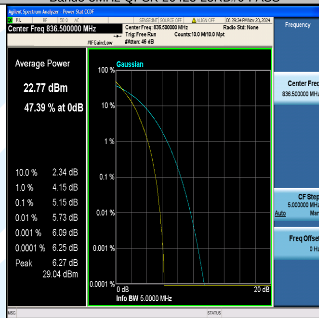
Band5-5MHz-QPSK-20525-25RB#0-PASS
