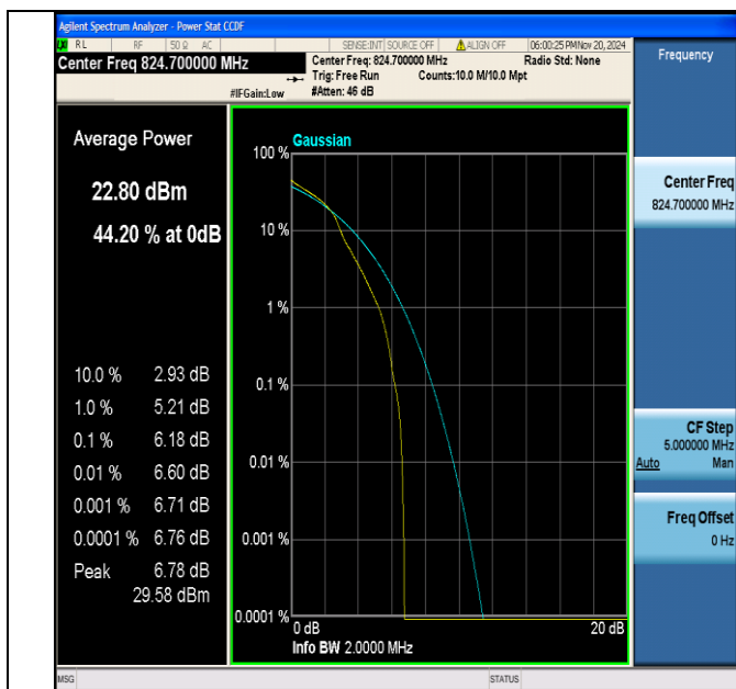
Band5-1.4MHz-16QAM-20407-1RB#0-PASS
