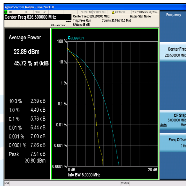
Band5-5MHz-QPSK-20425-25RB#0-PASS
