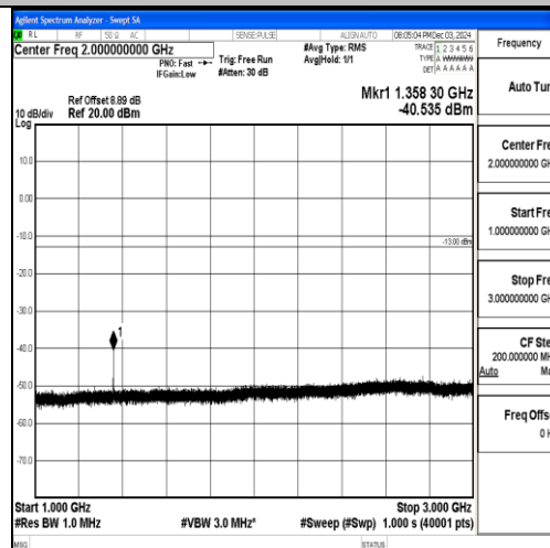
Band71_20MHz_16QAM_133372_1RB#0_1000~3000_1000~3000
