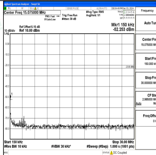
Band71_20MHz_16QAM_133372_1RB#0_0.15~30_0.15~30
