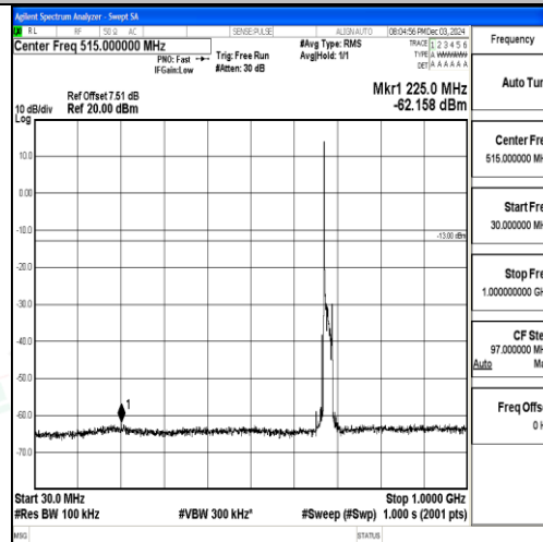
Band71_20MHz_16QAM_133372_1RB#0_30~1000_30~1000
