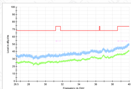
RSE-11AC-CH165-26.5GHz-40GHz
