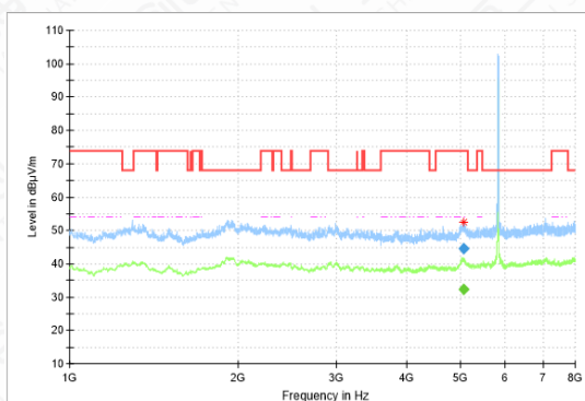
RSE-11AC-CH165-1GHz-8GHz
