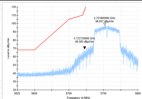
BANDEGE-11AC(40M)-CH151-PK
