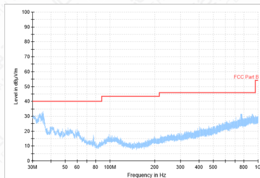
RSE-11AC(80M)-CH155-30MHz-1GHz
