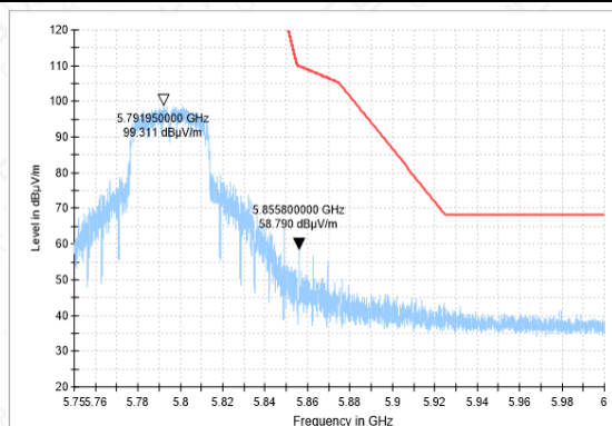
BANDEGE-11AC-CH157-PK
