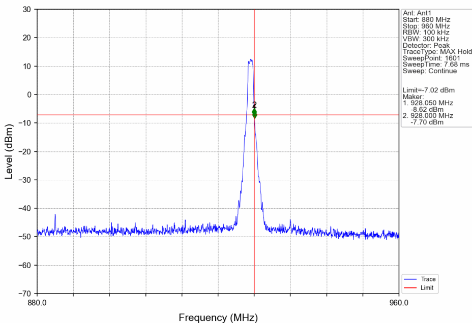
1.4M_HCH_927.2MHz_Ant1_NTNV
